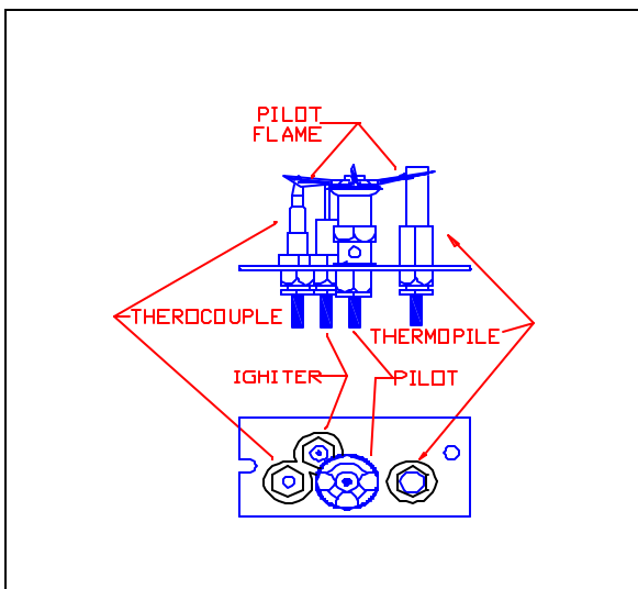
Figure 11: Pilot Adjustment
