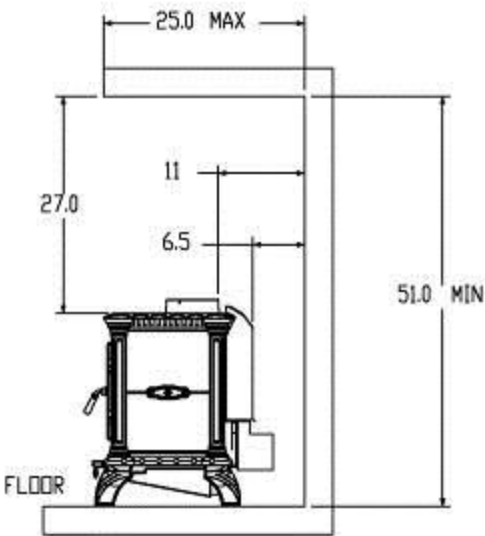
Figure 5: Tribute 8040 Allowable Minimum Alcove Clearances
