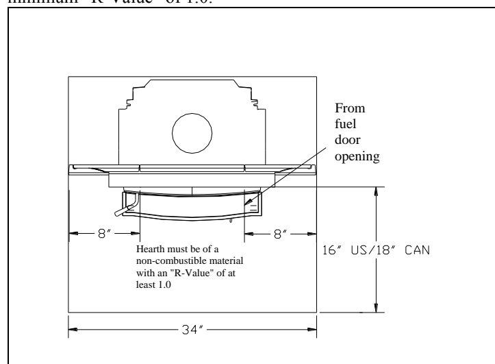
Figure 3 Hearth Requirements
