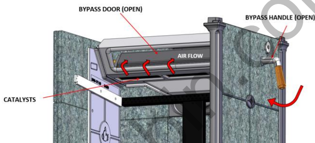
Figure 14 - Bypass Open
