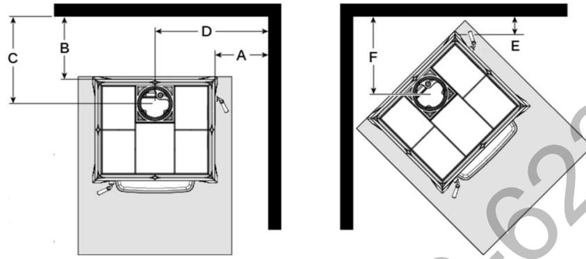
Figure 4 – Clearance to Combustibles
