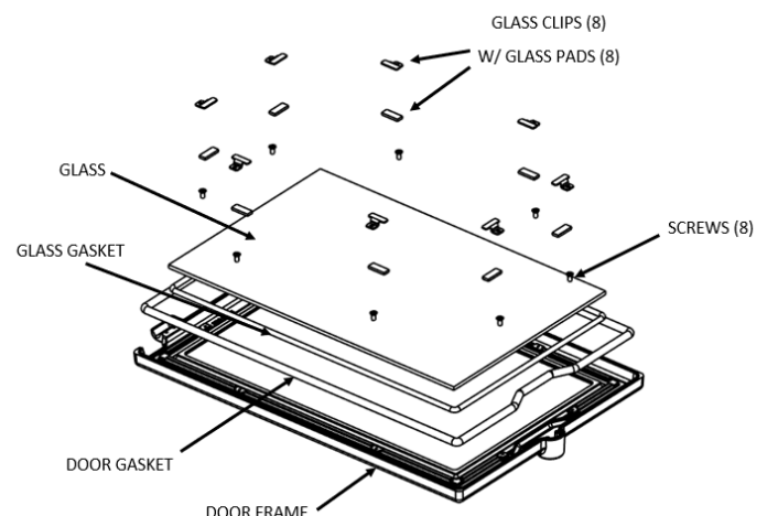
Figure 17 - Door assembly
