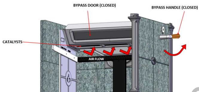
Figure 13 - Bypass Closed
