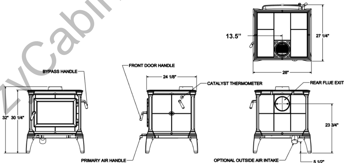
Figure 1 – Stove Dimensions
