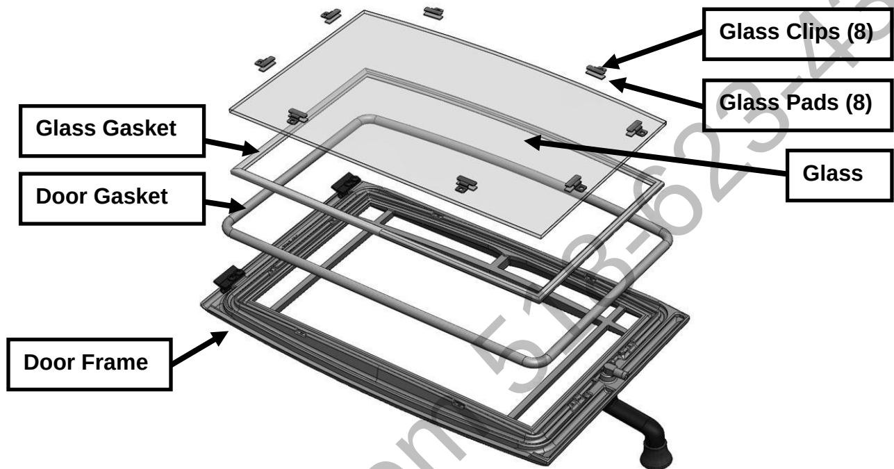
Figure 15: Front Door assembly
