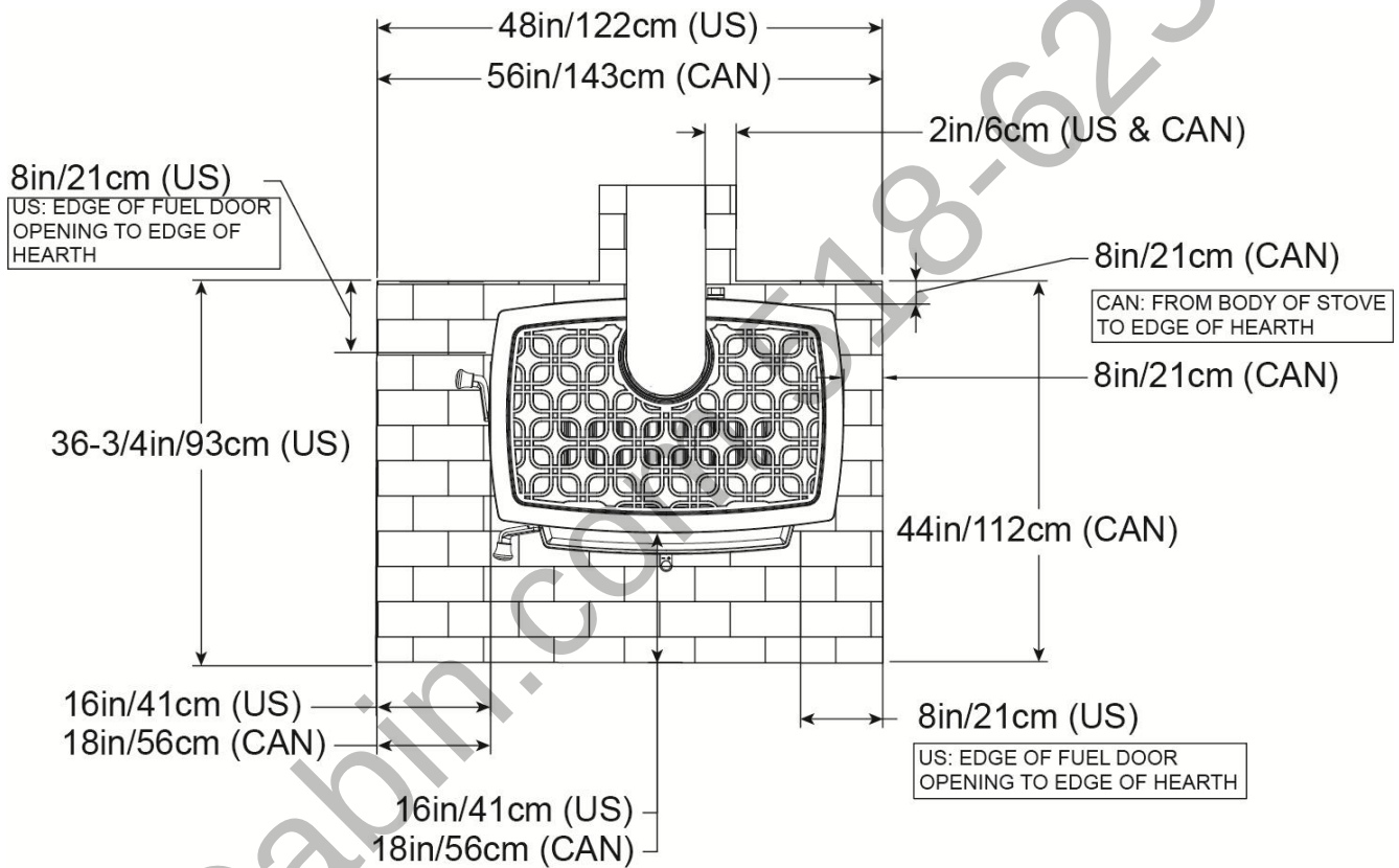
Figure 2 – Hearth Dimensions
