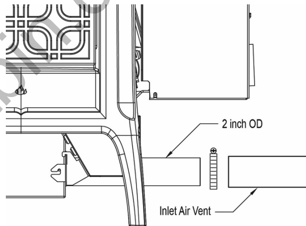
Figure 8 – Outside Air Attachment
