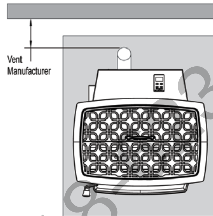
Figure 4 – Vertical Vent Clearance
