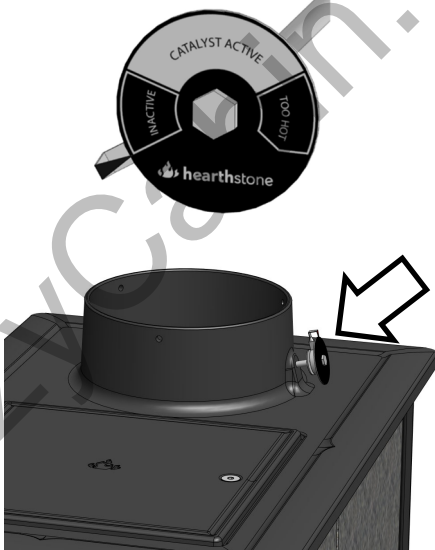
Figure 15 – Catalyst Thermometer
