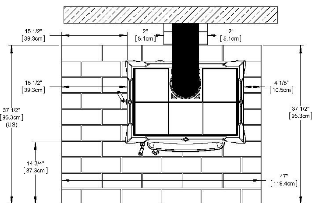
Figure 4 – Hearth Pad Dimensions
