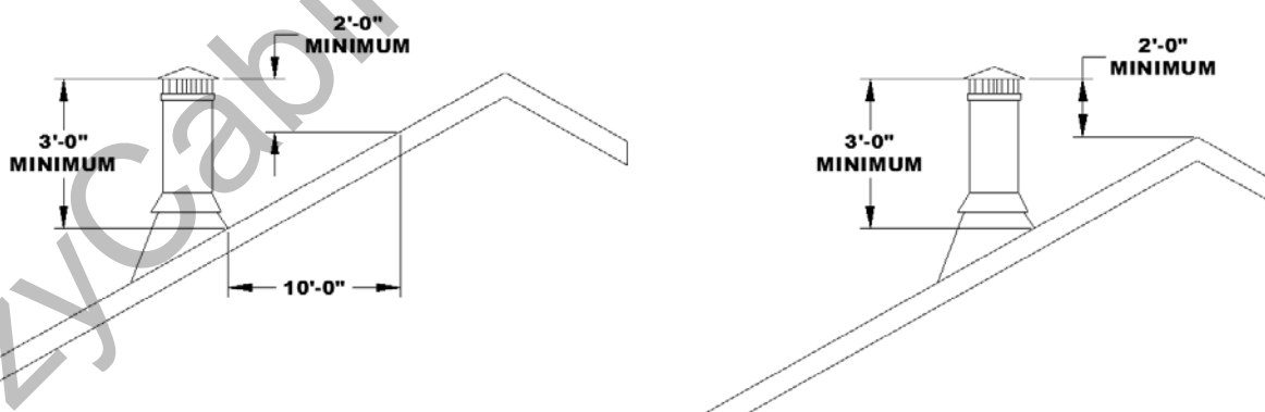
Figure 8 – Chimney Height Requirements
