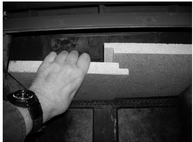
Figure 18 - Removing/Replacing the Baffle for Inspection
