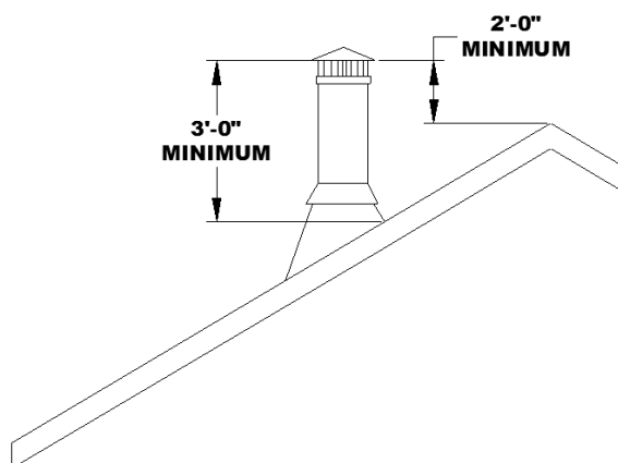
Chimney Height Requirements
