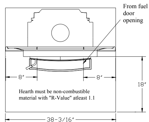
Figure 3 Hearth Requirements
