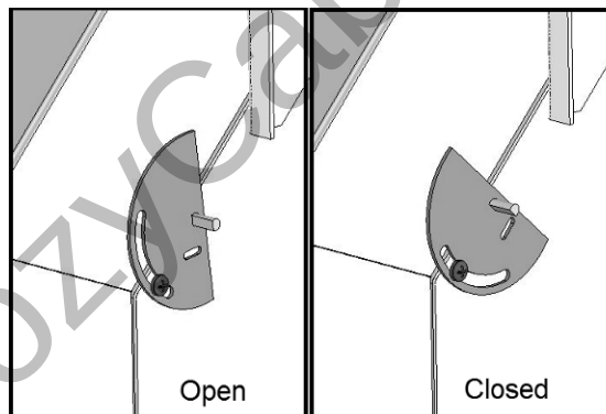
Figure 36 - Restrictor Adjuster Arm Detail
