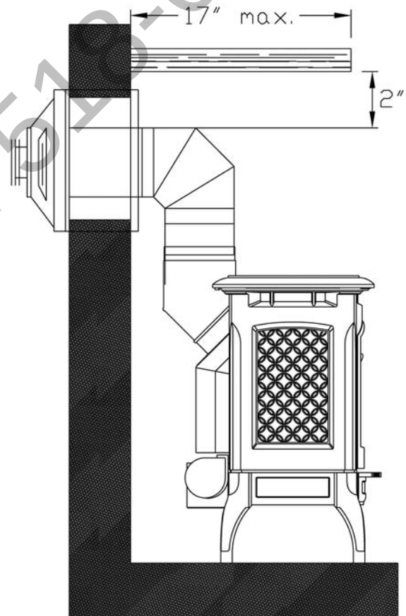
Figure 3: Mantle Clearance Horizontal Vent
