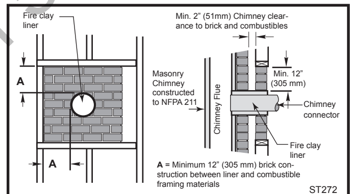
Fig. 7 Masonry Wall Pass-through with single wall chimney connector.
