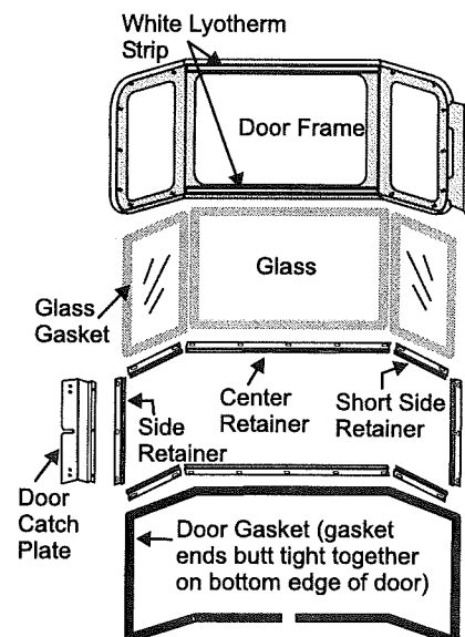
Panel Glass Door Assembly
