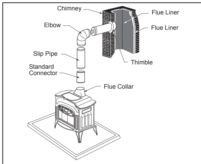
Figure 6 - Chimney connection is a freestanding installation.
