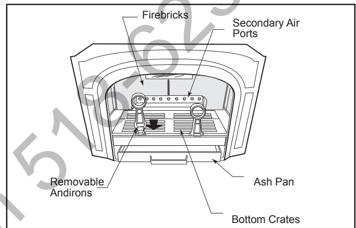
Figure 28 - A look inside the firebox of the Resolute Acclaim.
