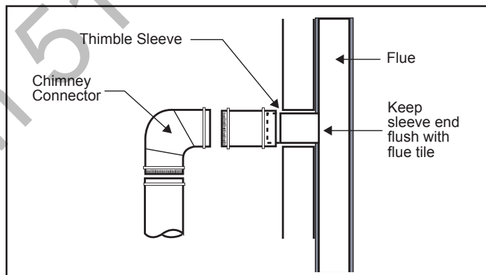
Figure 5 - The thimble, made of either ceramic or metal, must be cemented securely in place.
