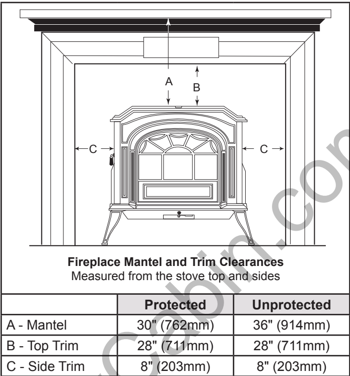
Figure 15 - Maintain clearances to combustible components of the mantelpiece.
