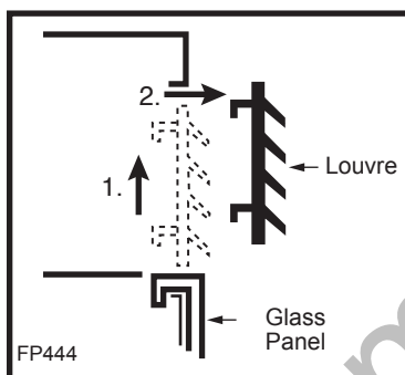
Fig. 15 Louvre removal.
