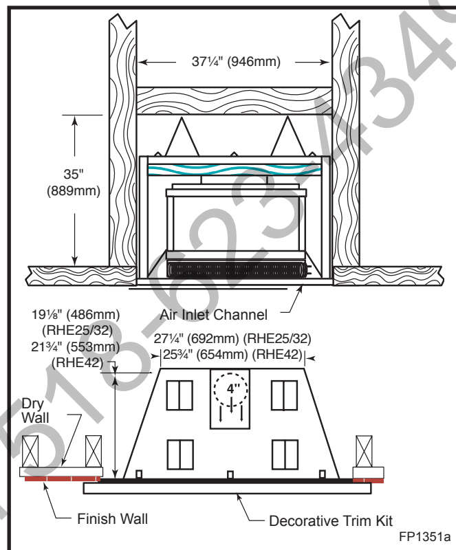
Fig. 3 RHE insert framing dimensions.
