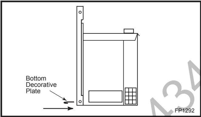
Fig. 47 Slide bottom decorative plate under unit floor.
