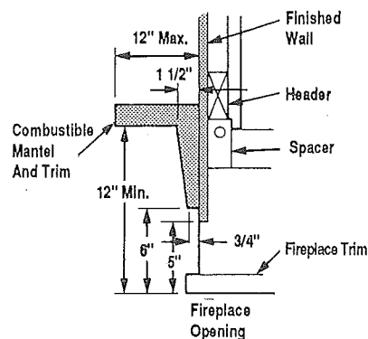
Typical Installation (Refer To Figure 50 For Canada)
