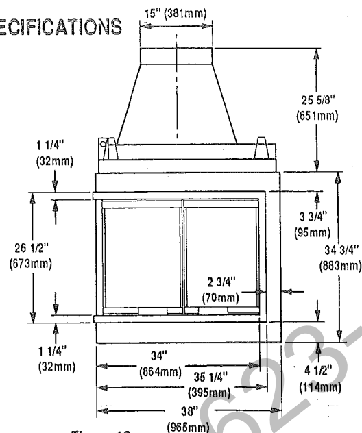
Figure 13 Front View
