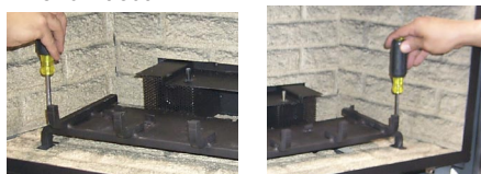
Diagram 1: Remove the left and right screws and then slide the burner/ grate assembly to the left and lift out.
