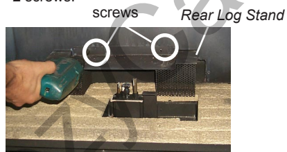
Diagram 1: Remove the left and right screws and then slide the burner/ grate assembly to the left and lift out.
