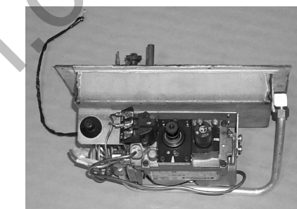
Diagram 1: Remove the left and right screws and then slide the burner/grate assembly to the left and lift out.
