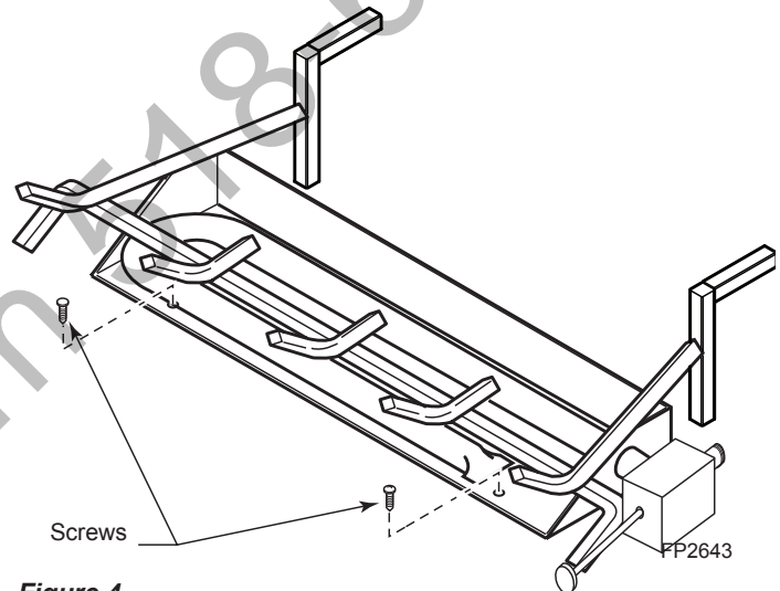
Figure 4 - Secure Grate/Burner Assembly into Firebox
