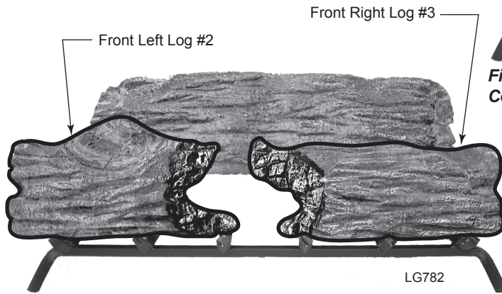
Figure 13 - Place Front Left Log #2 and Right Log #3
