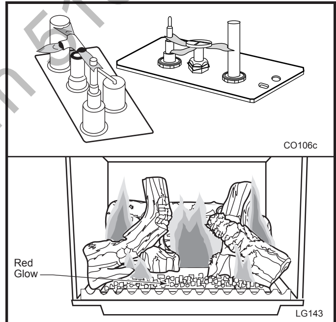
Fig. 47 Correct pilot and burner flame patterns.
