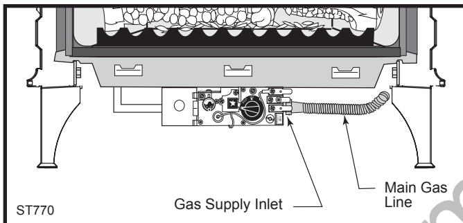
Fig. 48 Attach the gas line to the left side of the valve.
