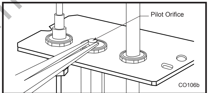
Fig. 55 Remove pilot orifice.
