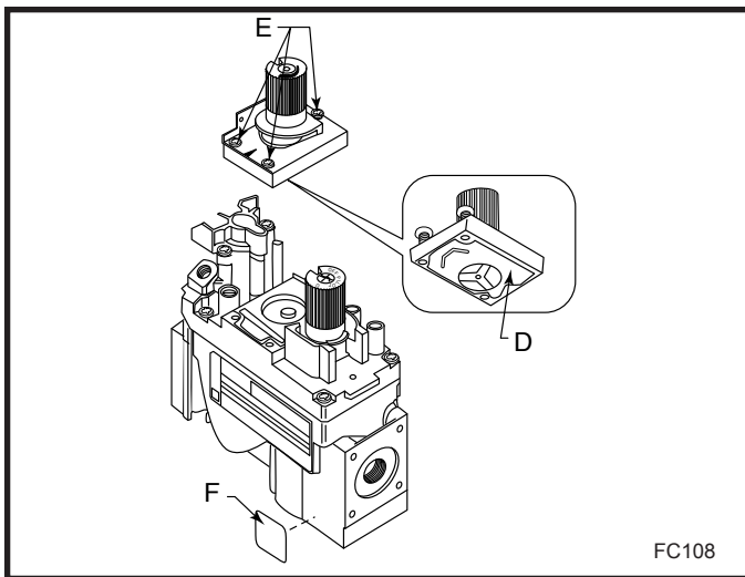
Fig. 51 Replace regulator.
