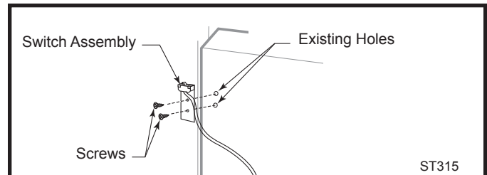
Fig. 41 Attach switch assembly to rear shroud.
