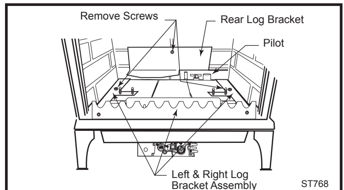
Fig. 37 Remove rear log bracket and left and right log bracket assembly.
