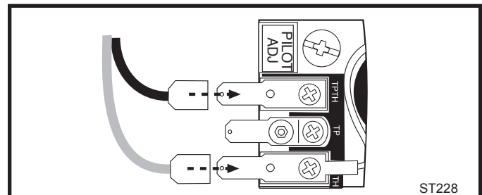
Fig. 42 Attach switch wires to valve.
