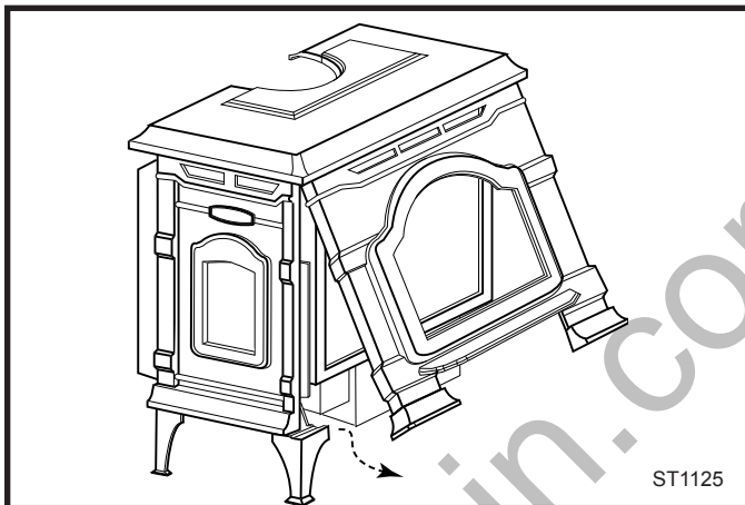
Fig. 57 Remove the stove front.
