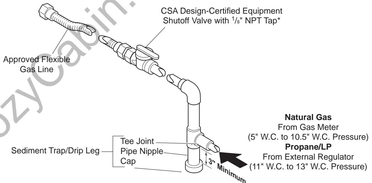
Figure 32 - Gas Connection
