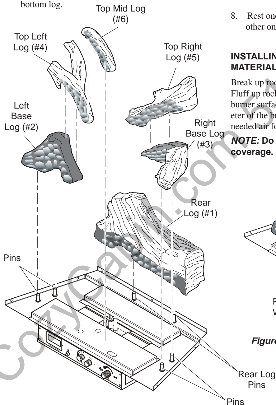
Figure 39 - Installing Logs on Base (CSDV40)
