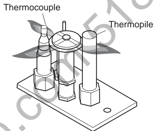
Figure 47 - Typical Pilot Flame (CSDV20 and CSDV30)
