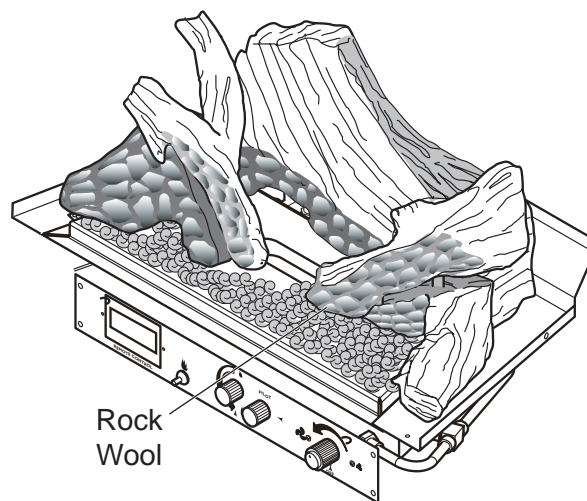
Figure 38 - Installing Rock Wool (CSDV30)
