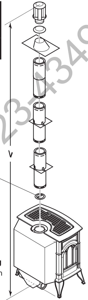
Figure 30 - Vertical Rigid Venting Configuration with No Horizontal run
