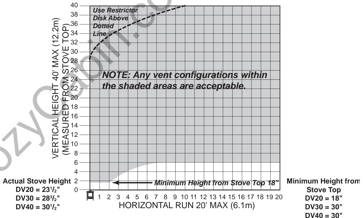
Figure 11 - Acceptable Vent Configurations
