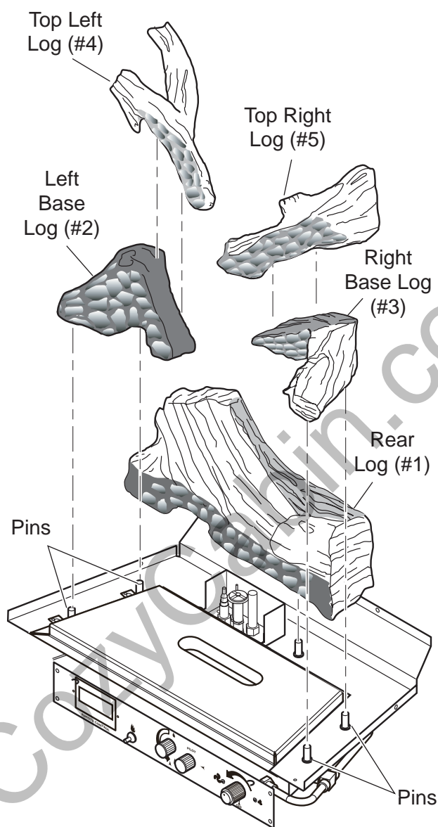
Figure 37 - Installing Logs on Base (CSDV30)
