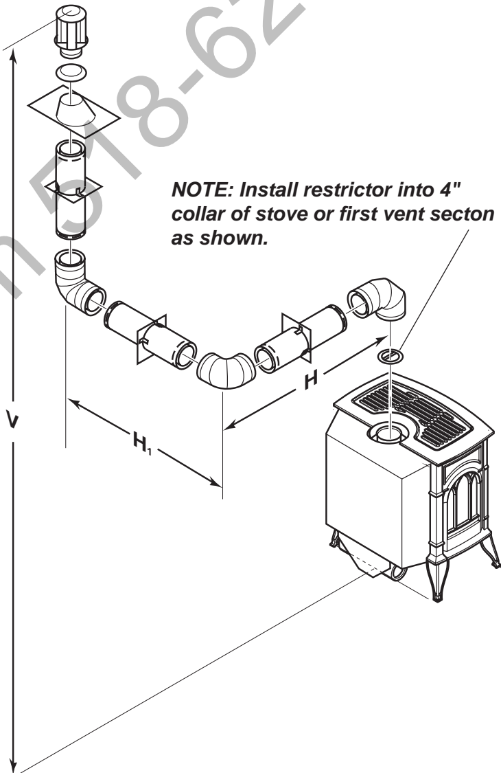
Figure 28 - Vertical Rigid Venting Configuration Using Three 90° Elbows with Two Horizontal Runs
