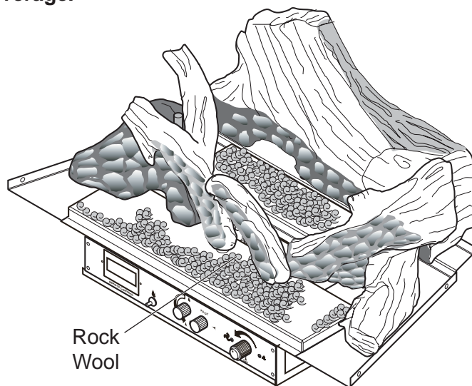
Figure 40 - Installing Rock Wool (CSDV40)
