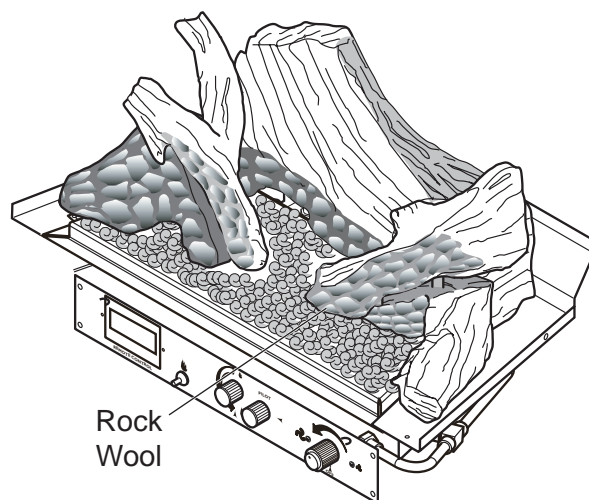
Figure 36 - Installing Rock Wool (CSDV20)
