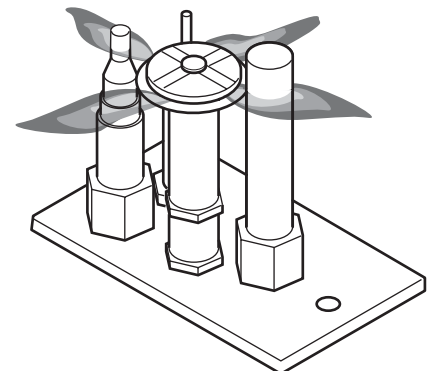
Figure 48 - Typical Pilot Flame (CSDV40)
