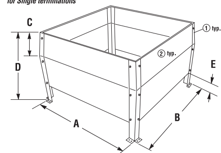
CTSO-33/44 Shrouds for single terminations
