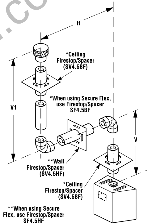
Figure 29 - Top Vent - TWO 90 DEGREE ELBOWS
