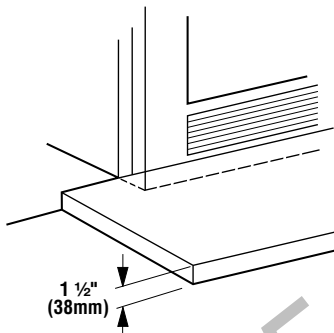
Max. Thickness of Hearth Extension when LBC Models are on the Floor
