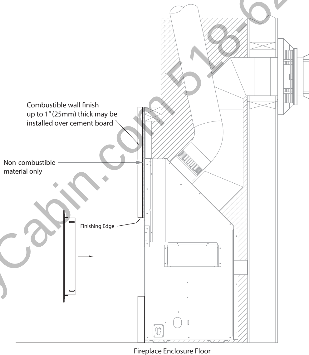
Figure 3.4, KZK-158A Combustible Wall Finish with Surround
