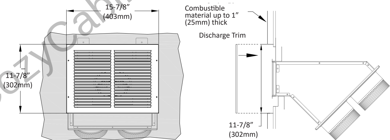
Figure 3.5 - KZK Air Discharge Grille Finishing Trim
