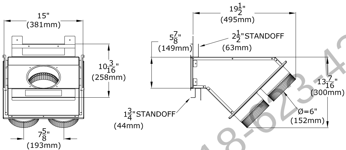
Figure 1.4 - KZK-1510 Plenum Dimensions
