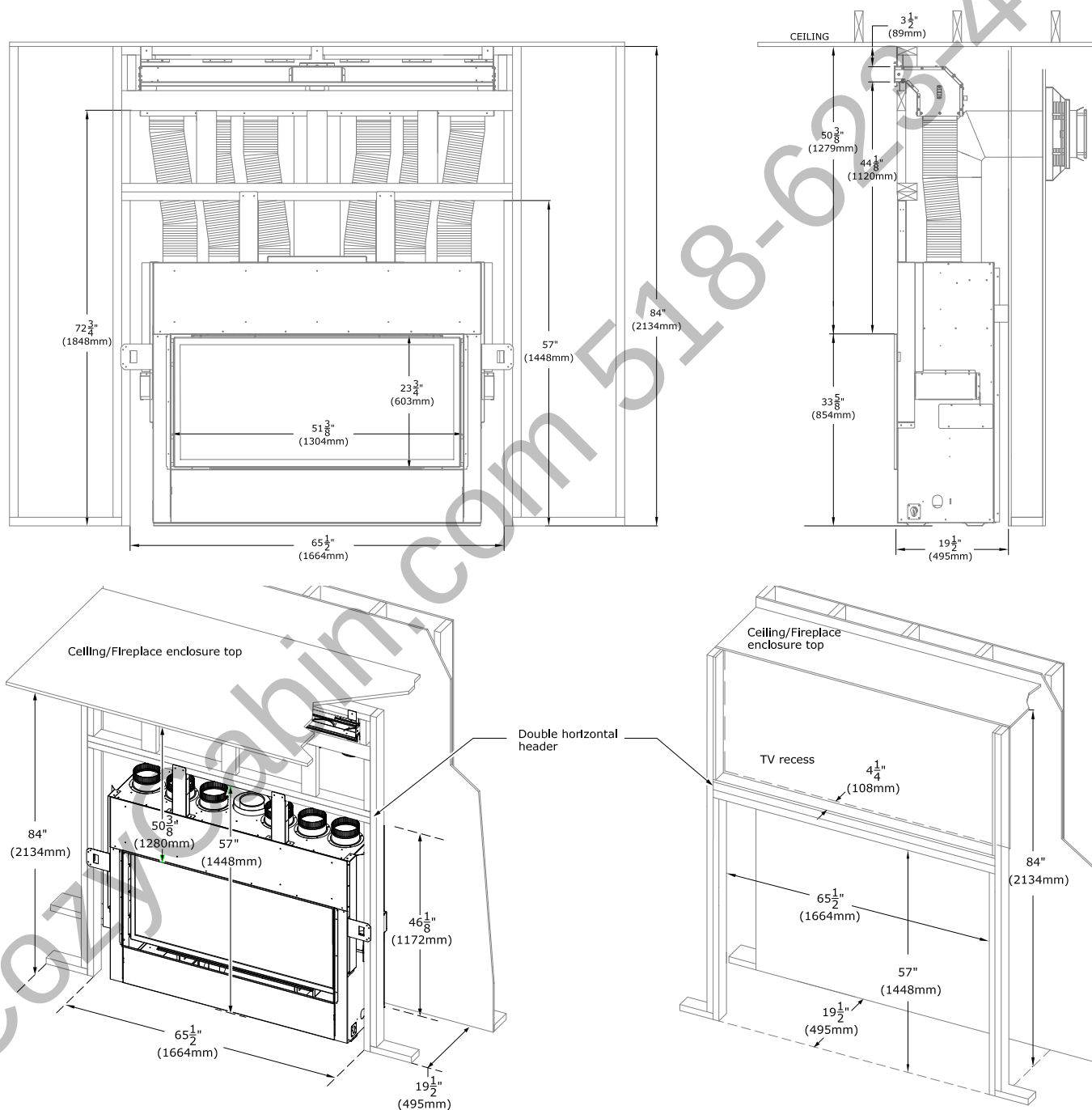
Figure 2.5 - Nordik 48TL Plenum Framing
