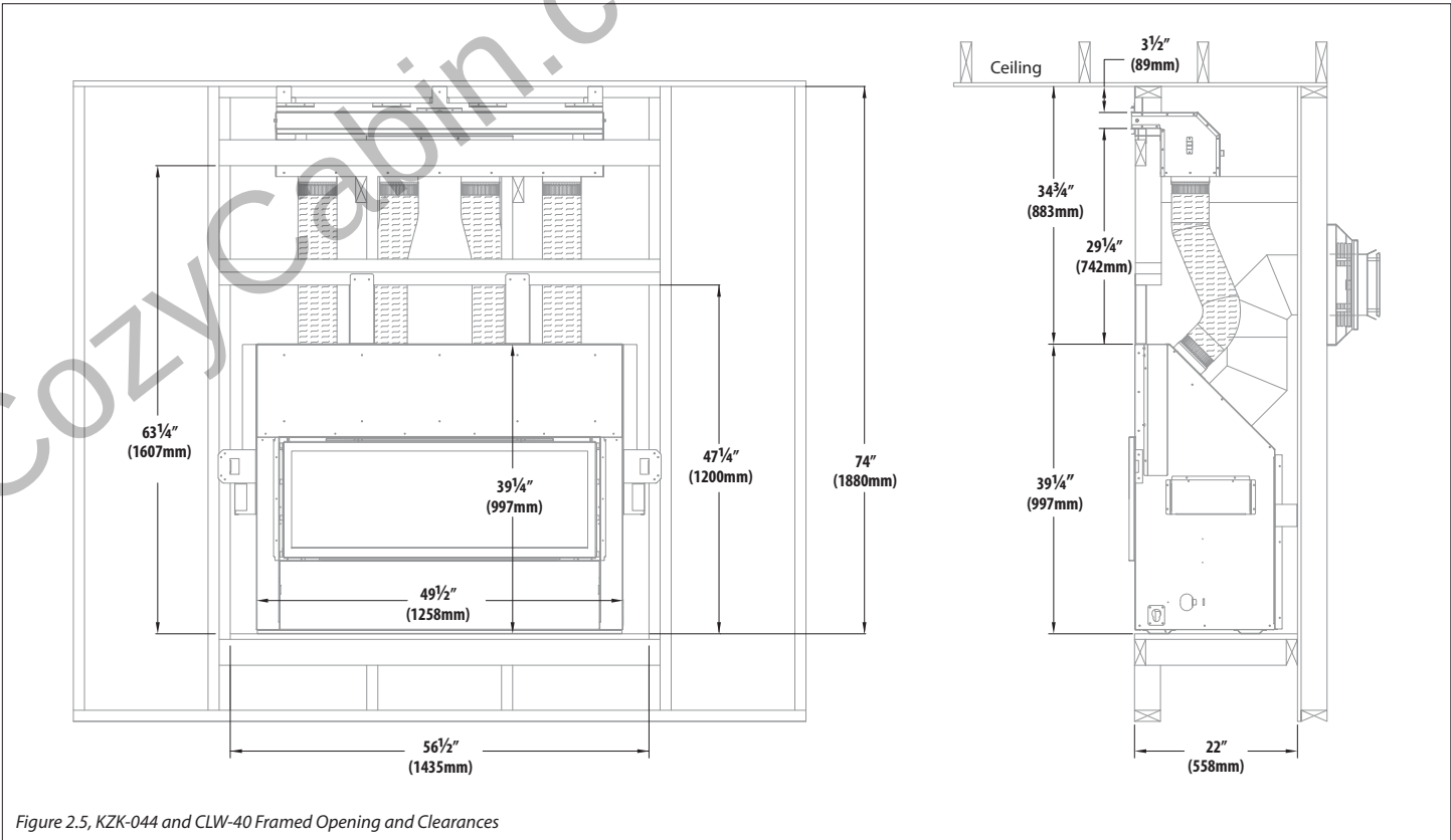
Figure 2.5, KZK-044 and CLW-40 Framed Opening and Clearances
