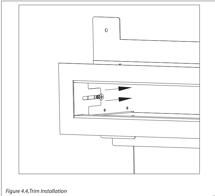
Figure 4.4, Trim Installation
