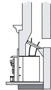
1) Positive Flue Connection with Cleanout
