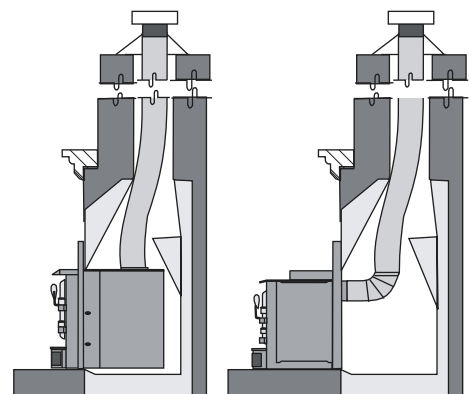
Flush Inserts
