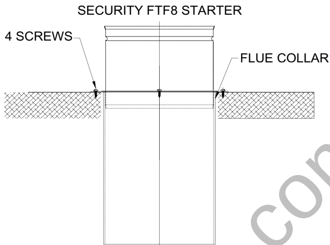
Security FTF8 Chimney System
