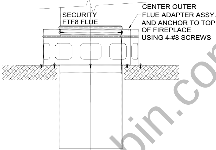
Security FTF8 Chimney System
