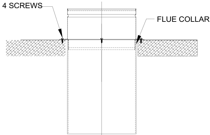
Majestic SK8 Chimney System
