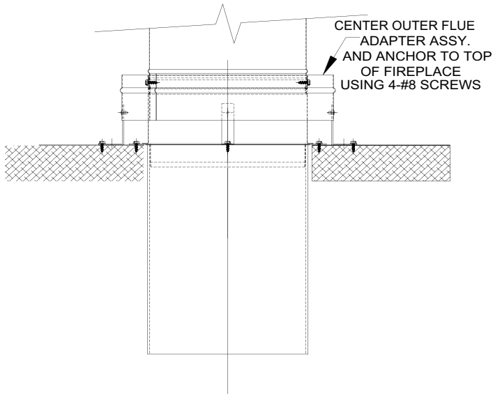
Majestic SK8 Chimney System
