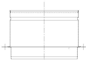
INNER FLUE ADAPTER FOR MAJESTIC SK8 SERIES CHIMNEY
