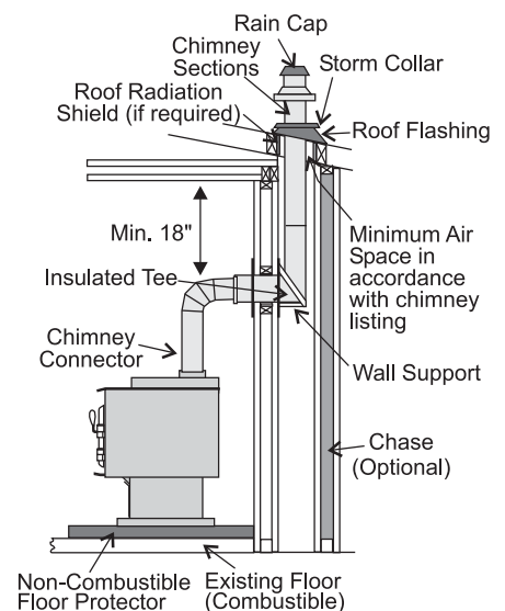
Horizontal Installation
