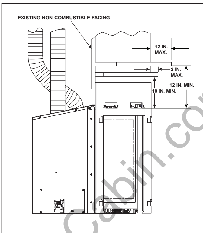
Figure 10.1 Mantel Clearance
