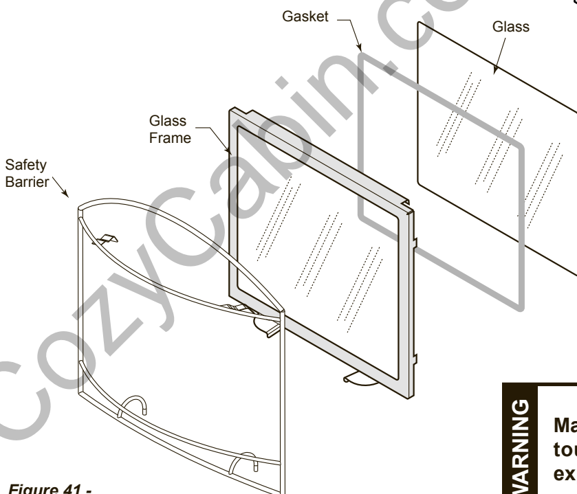
Figure 41 - Glass Replacement
