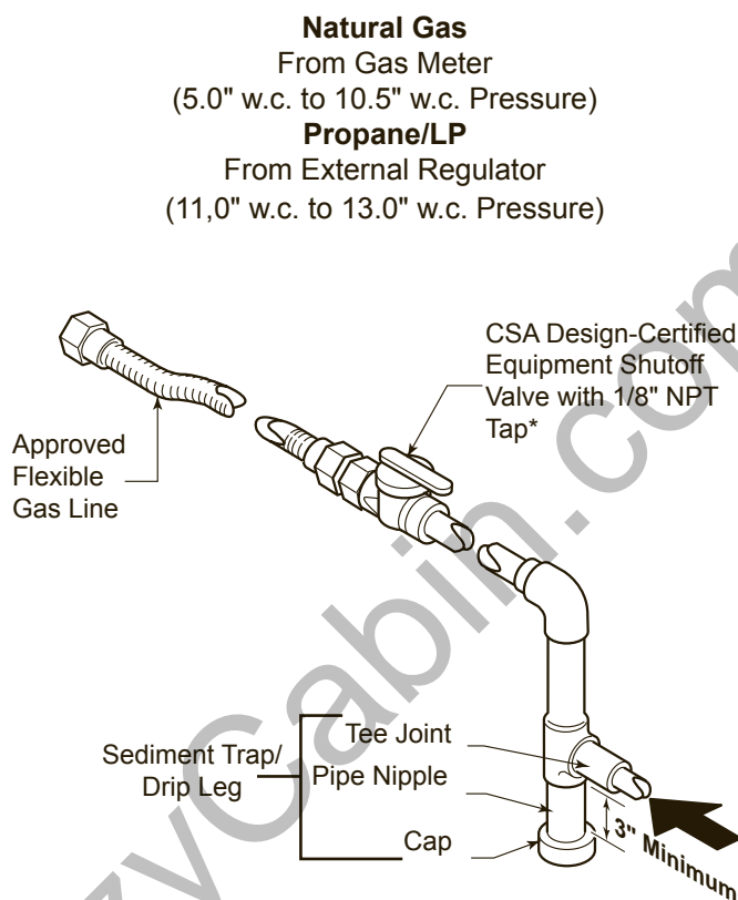
Figure 31 - Gas Connection
