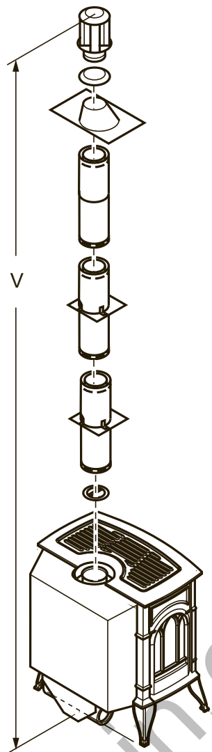
Figure 29 - Vertical Rigid Venting Configuration with No Horizontal Run
