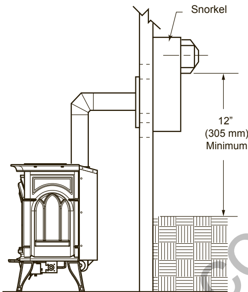
Figure 12 - Snorkel Termination
