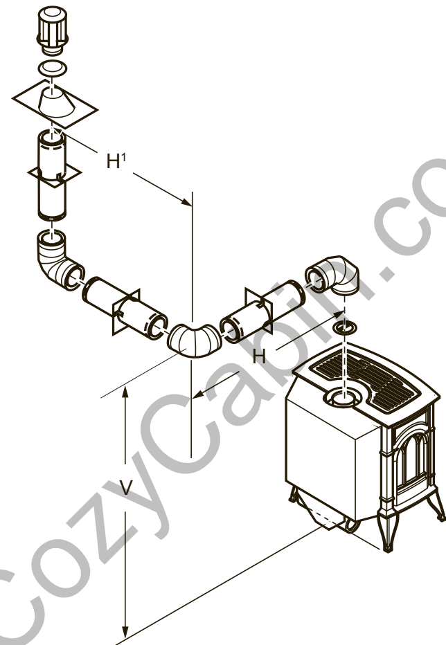
Figure 27 - Vertical Rigid Venting Configuration using Three (3) 90° Elbows with Two (2) Horizontal Runs
