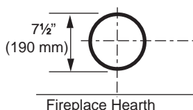
Figure 31 - Locate vent opening on wall
