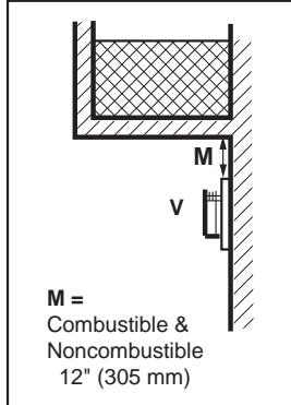
Figure 17 - Termination Clearances
