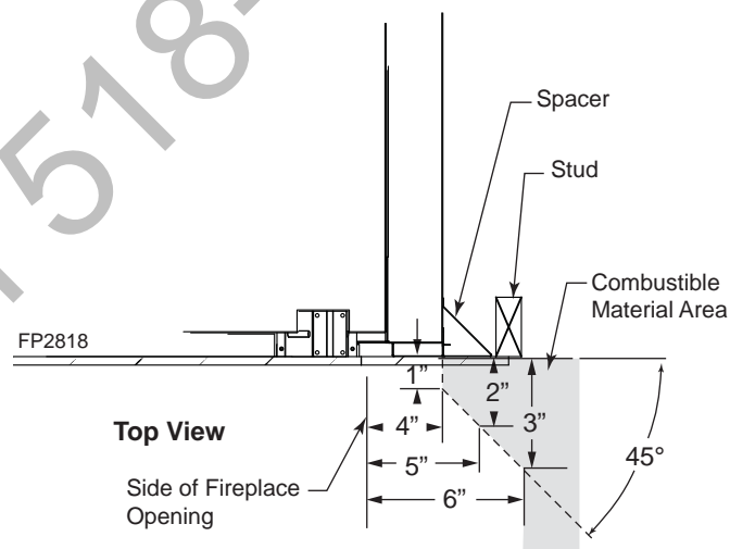
Figure 10 - Mantel Clearance
