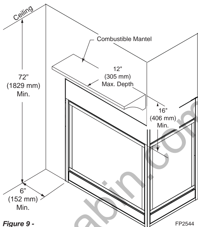
Figure 9 - Ceiling and Side Wall Clearances
