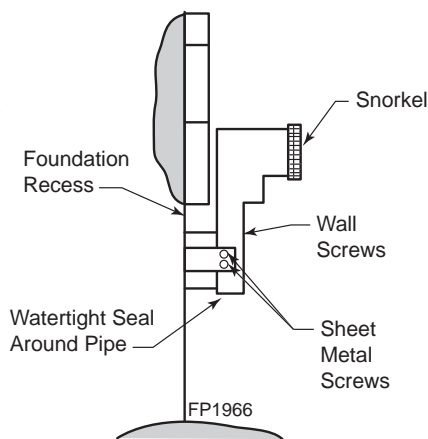
Figure 33 - Snorkel Installation, Recessed Foundation
