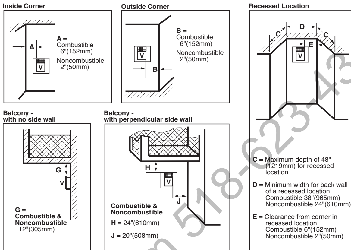
Fig. 13 Termination clearances.
