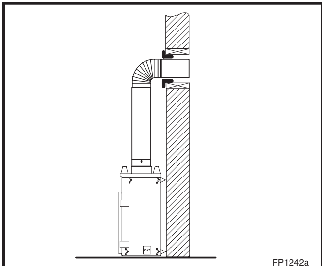
Fig. 25 Through the wall.
