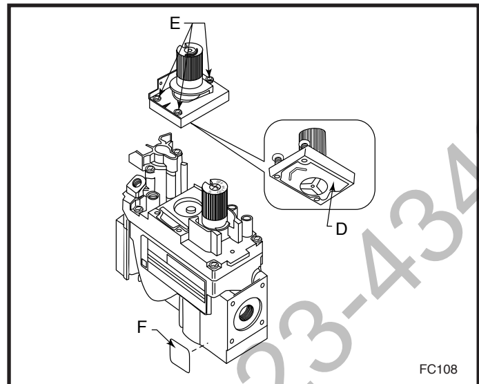
Fig. 57 Replace regulator.
