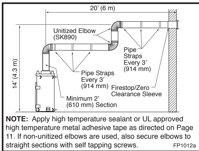
Fig. 17 Support straps for horizontal runs.
