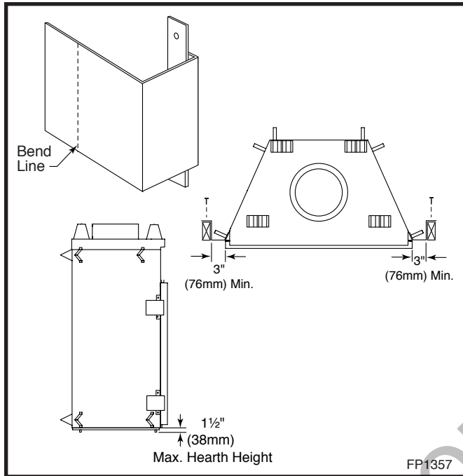
Fig. 5 Nailing flanges.
