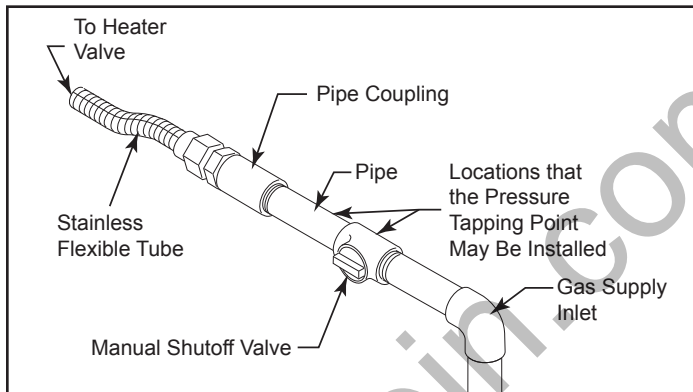
Figure 9 - Gas Connection
