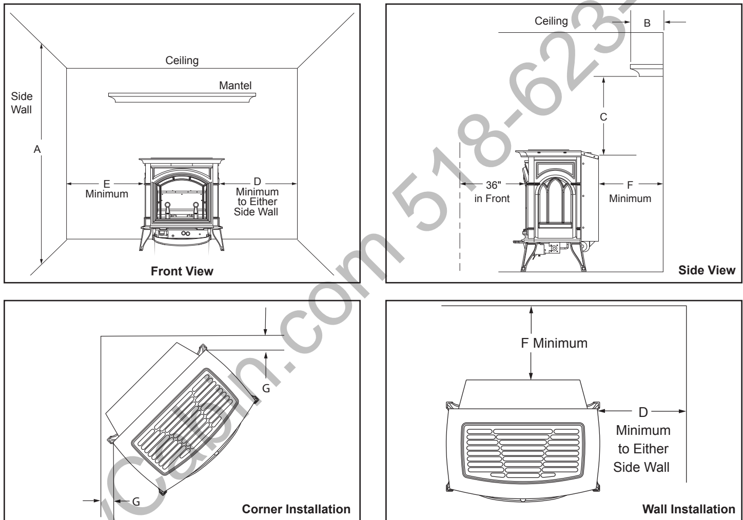
Figure 4 - Minimum Clearances
