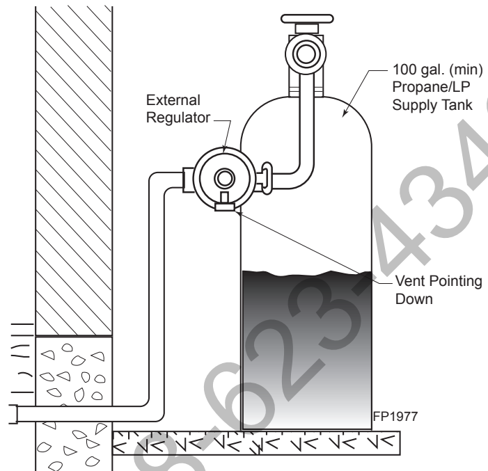
Figure 32 - External Regulator with Vent Pointing Down (Propane/LP Only)
