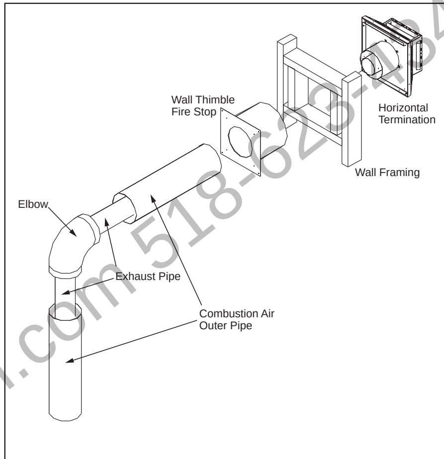
Figure 66: Horizontal Vent Termination
