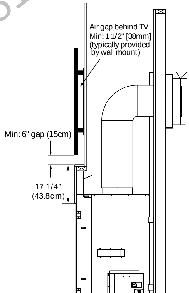
Figure 59: Recess Minimum TV Install
