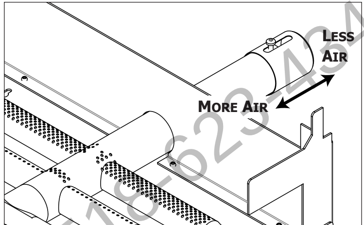
Figure 12: Burner Shutter Adjustment
