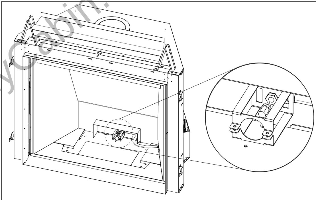
Figure 22: Orifice Location
