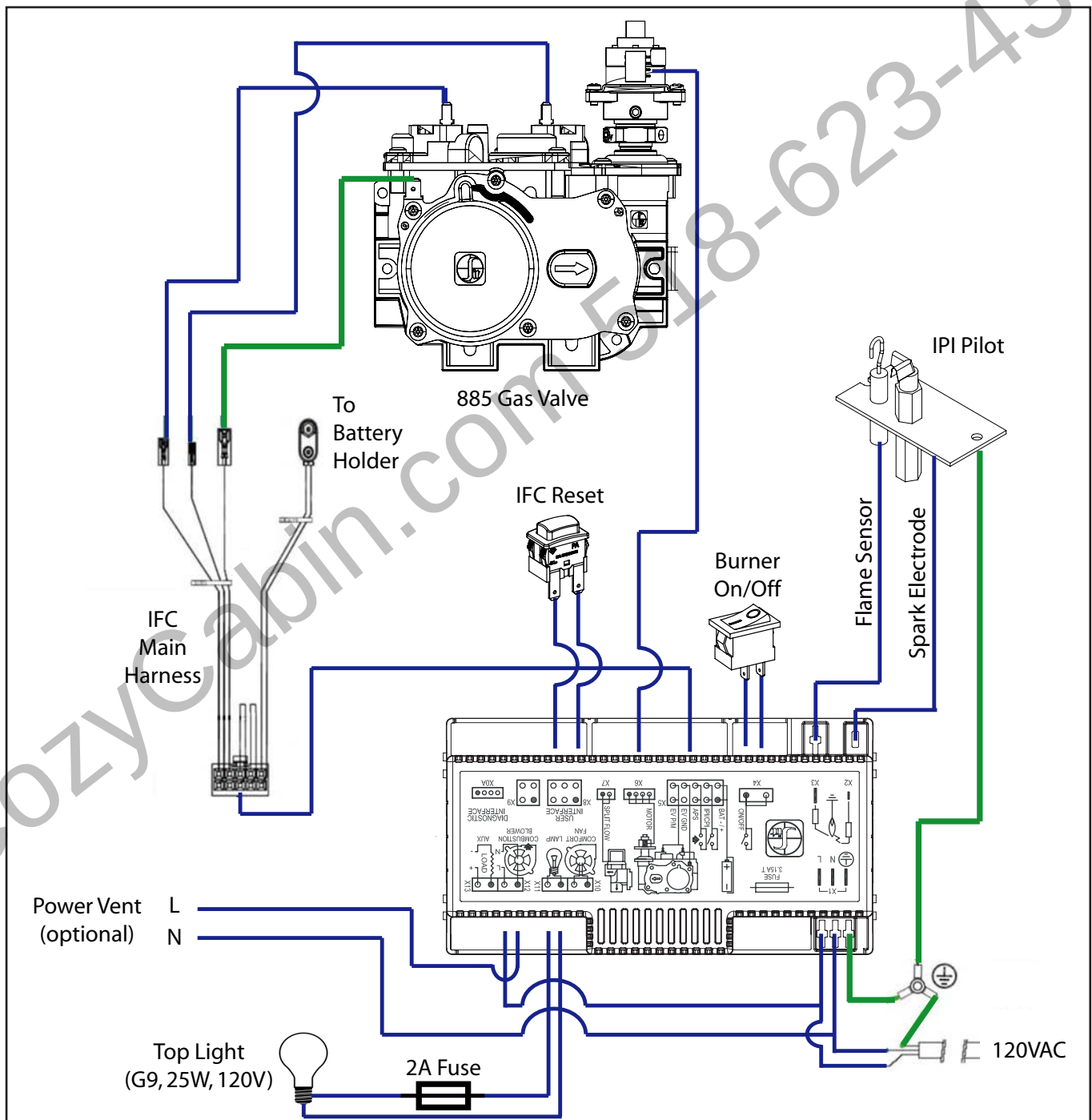
Figure 72: Wiring Diagram
