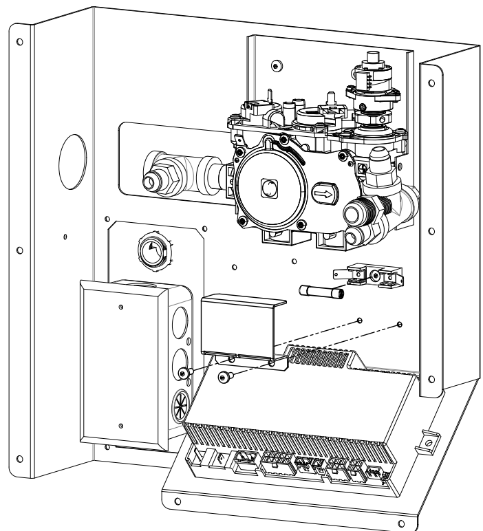
Figure 21: Fuse Removal
