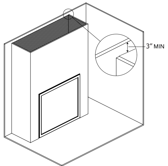
Figure 45: Open Chase Iso View
