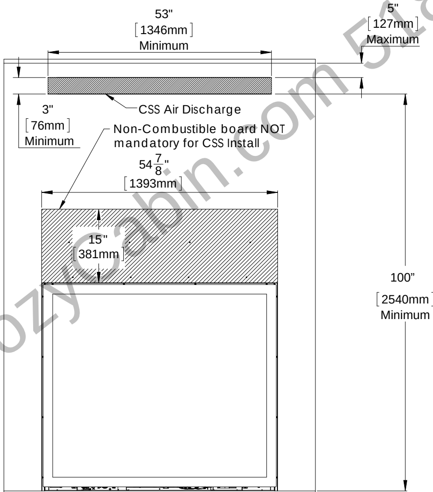
Figure 41: Framing Option 1
