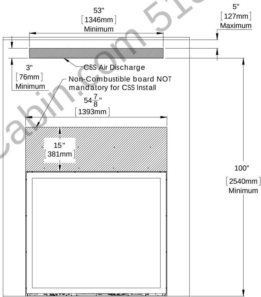
Figure 57: Typical Facing Layout
