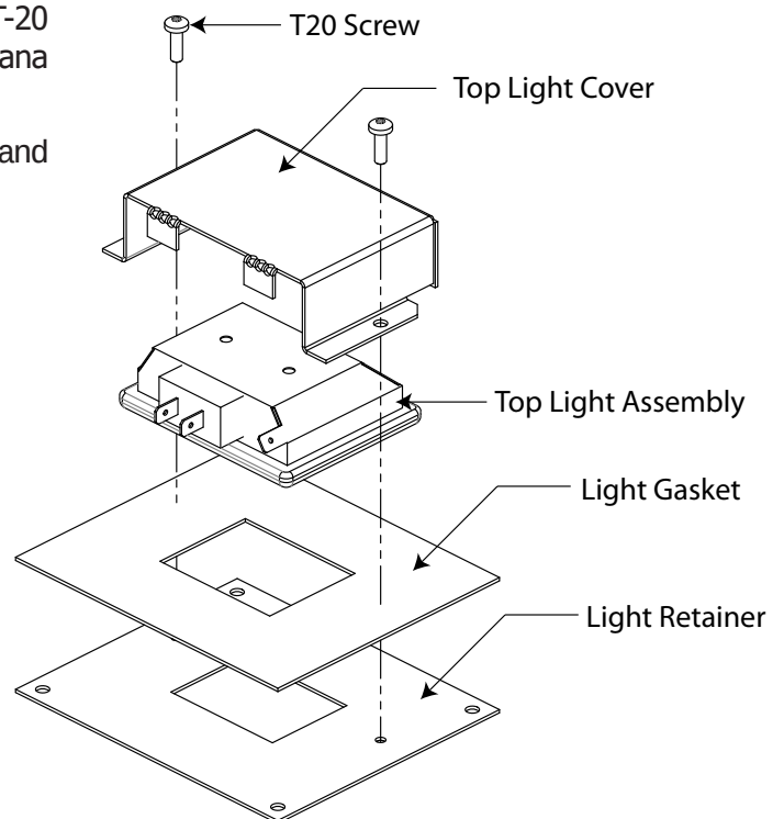
Figure 16: Top Light Assembly
