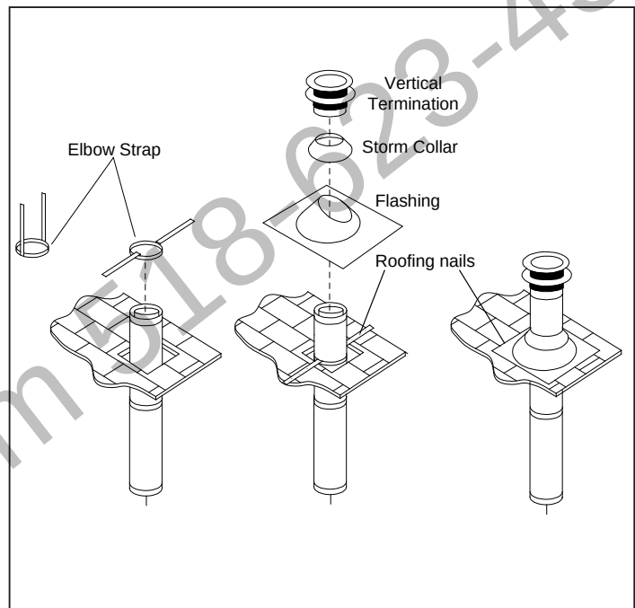
Figure 67: Vertical Vent Termination
