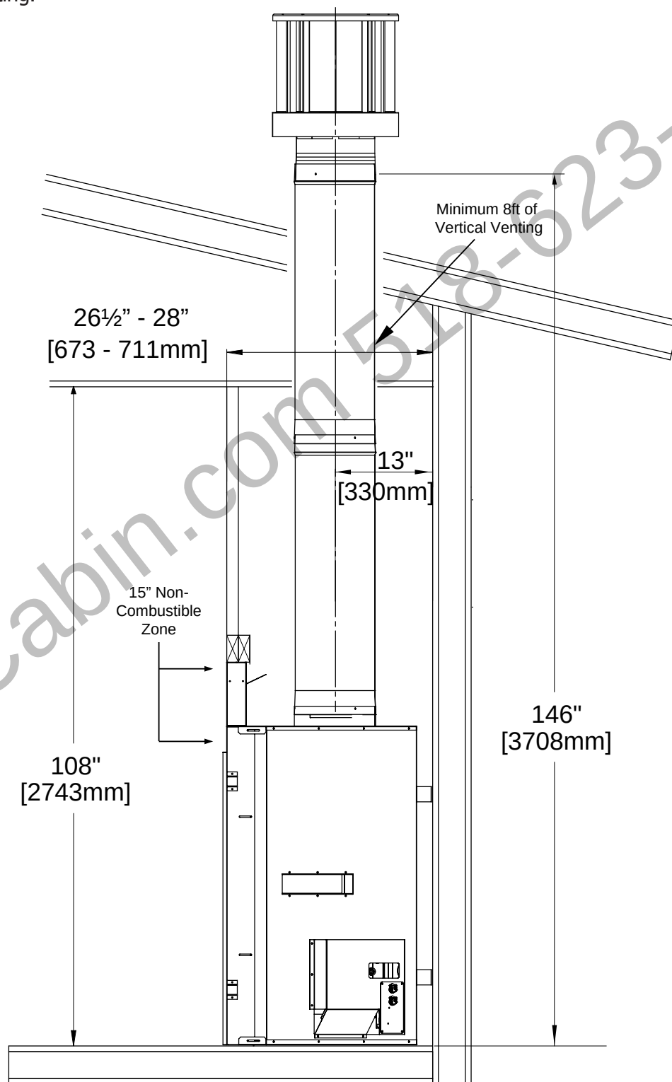
Figure 56: Minimum Vent for Propane [LP]
