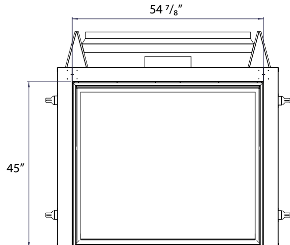
Figure 38: Finishing Edge Dims
