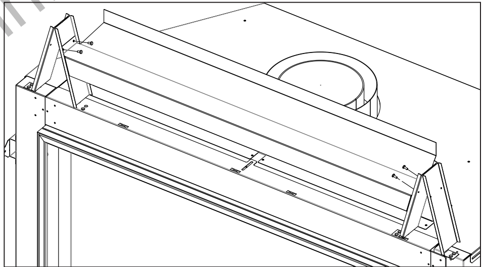
Figure 32: Top Standoff Support Install
