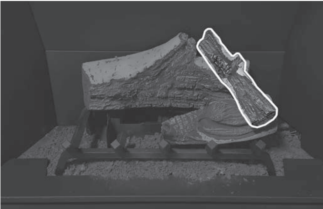
Figure 77: Log Set Installation - Step 3
