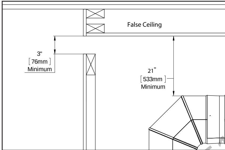
Figure 42: False Ceiling
