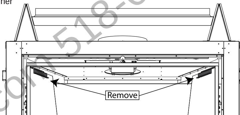
Figure 74: Liner Retainers
