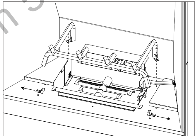
Figure 9: Log Grate Removal
