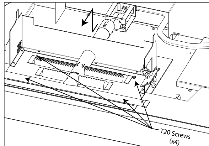
Figure 11: Log Burner Removal
