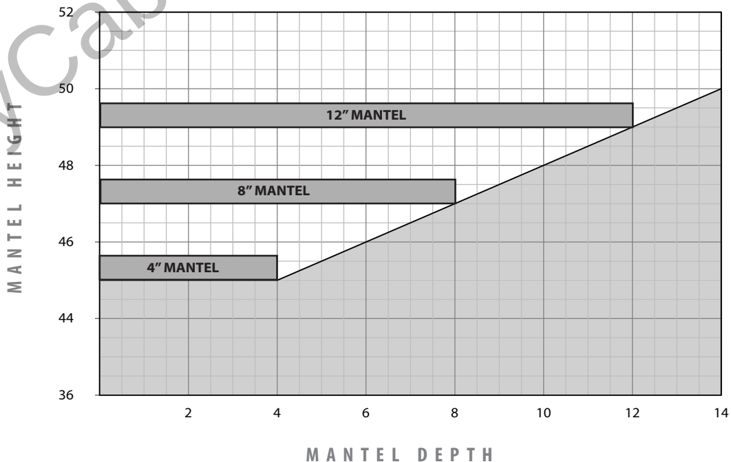
Figure 54: Mantel Clearances - CSS Activated
