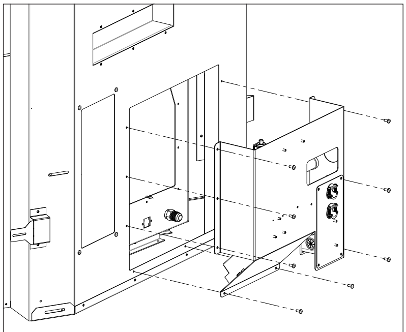
Figure 13: Component Backpack Removal
