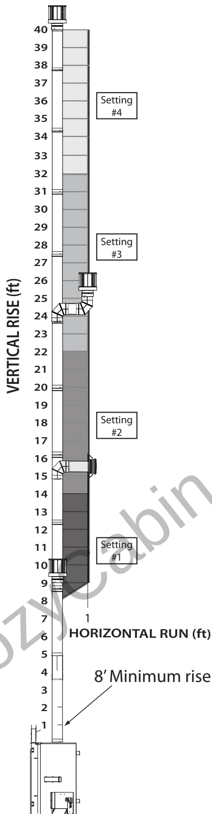
Figure 63: 8" x 11" LP Vent Graph
