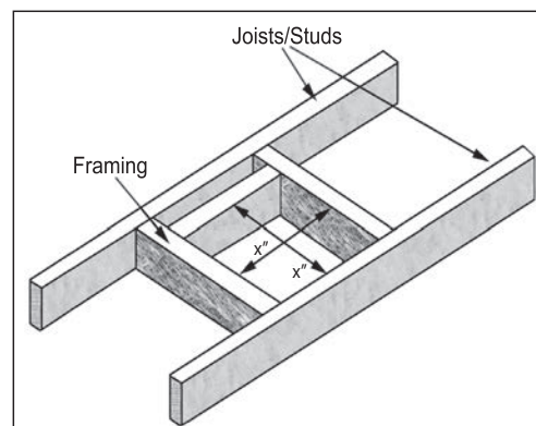
Figure 61: Thimble Framing
