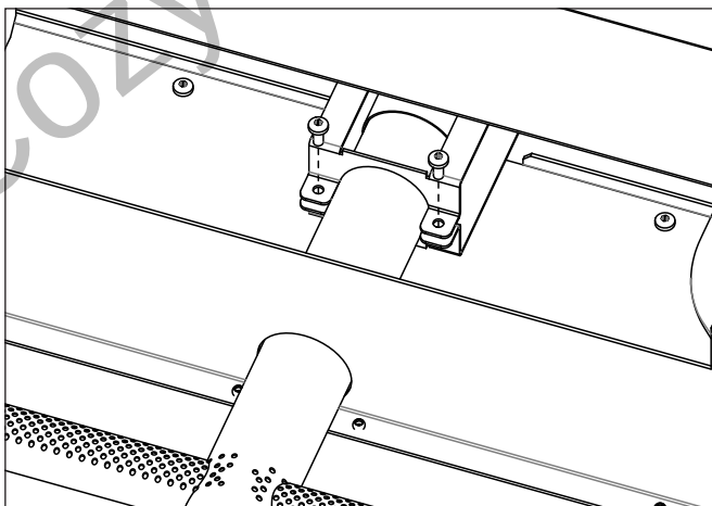
Figure 10: Orifice Mount Clamp
