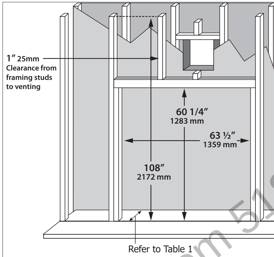
Figure 37: U55 Minimum Framing
