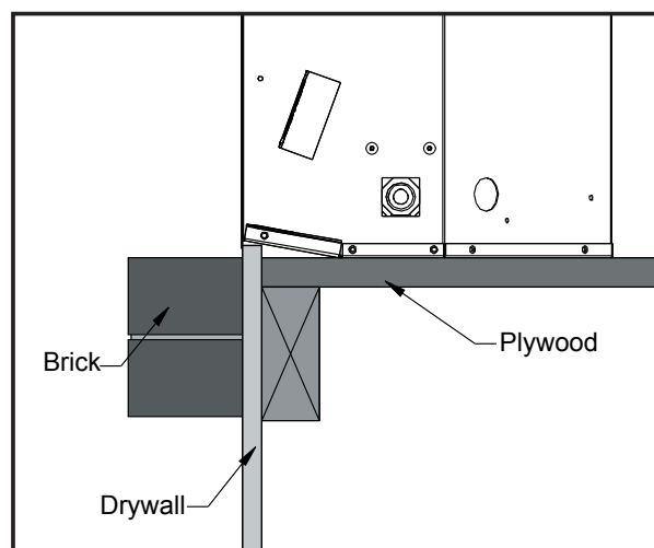
Figure 27. Drywall & Brick Facing Around The Retreat.
