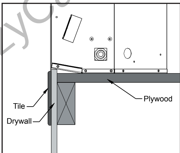
Figure 26. Drywall & Tile Facing Around The Retreat.
