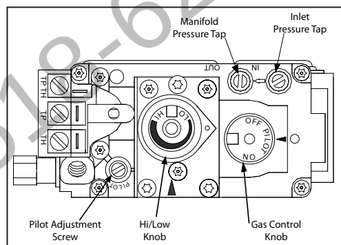
Figure 45. Fully Labeled Gas Valve.
