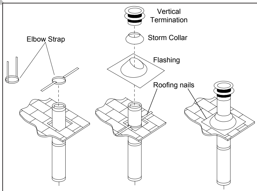
Figure 39. Vertical Vent Termination
