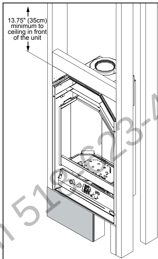
Figure 22. Raised Fireplace with No Hearth.
