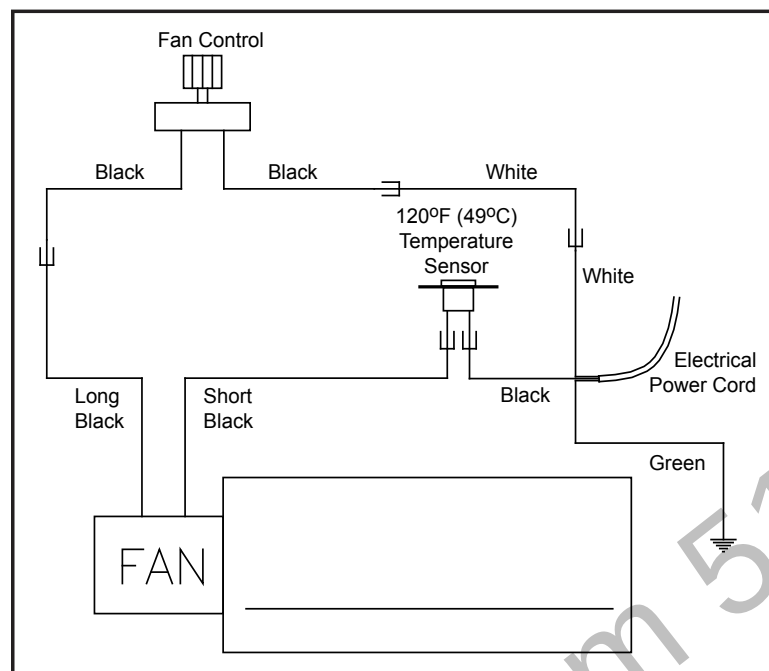
Figure 46. Wiring Diagram For Fan Control.
