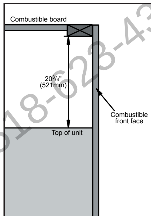
Figure 29. Combustible Shelf Clearance
