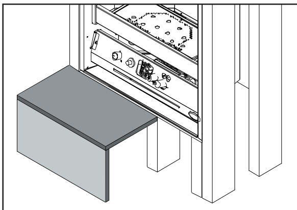
Figure 20. Raised Fireplace with Raised Hearth.
