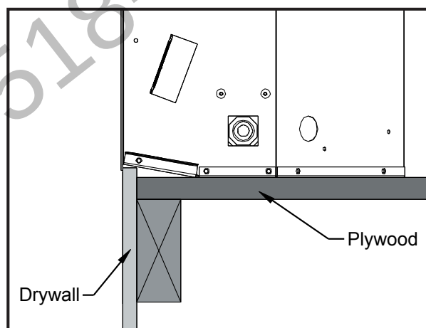
Figure 25. Drywall Facing Only Around The Retreat.
