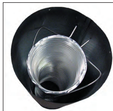
Figure 32: Wire Spacer in Place.
