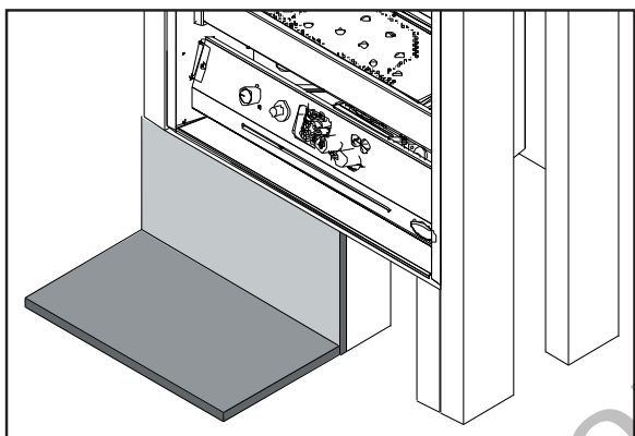
Figure 21. Raised Fireplace with Floor Level Hearth.
