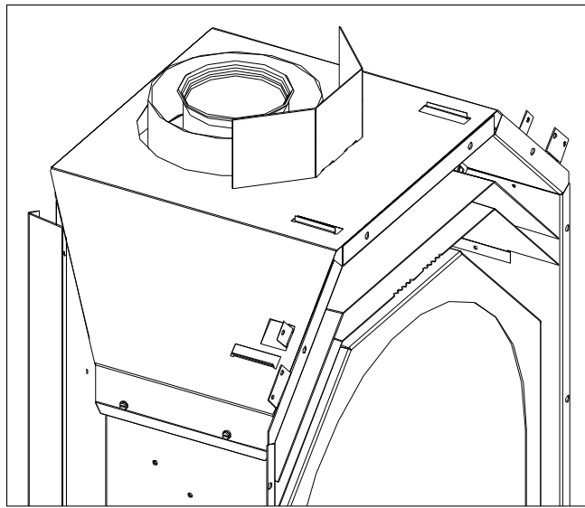
Figure 11. Vent Heat Shield Sides Bent.
