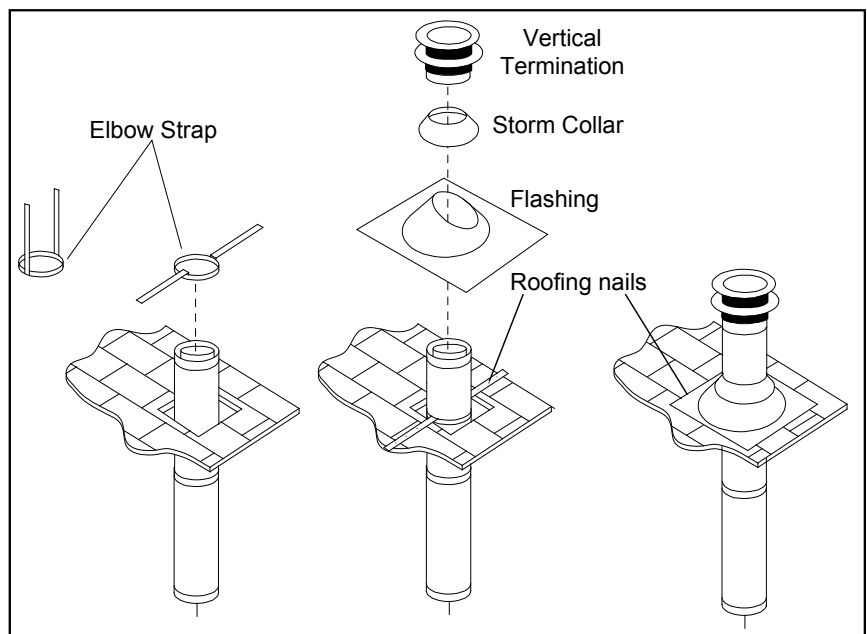
Figure 34. Vertical Vent Termination
