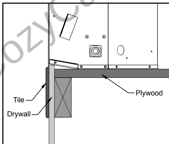
Figure 21. Drywall & Tile Facing Around The Retreat.
