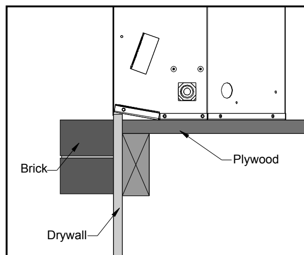
Figure 22. Drywall & Brick Facing Around The Retreat.
