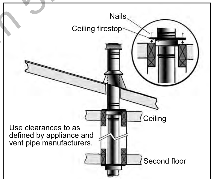
Figure 37. Multi-Story Vent Pipe Installation.
