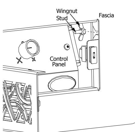
Figure 57: Fastening Bottom of Chalet.
