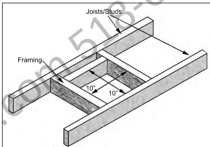
Figure 30. Vent Framing Through the Wall or Ceiling.
