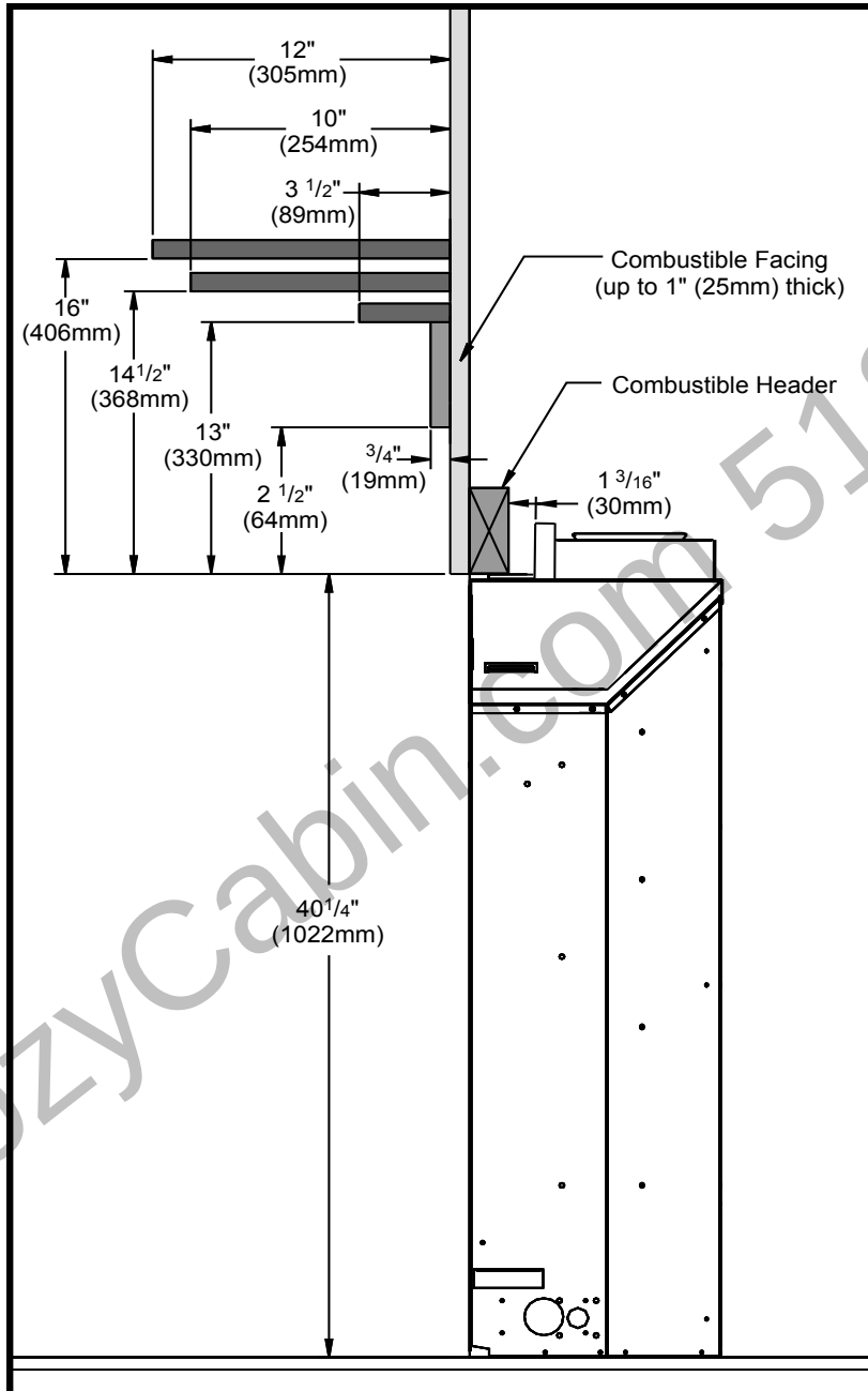
Figure 23. Combustible Mantle Clearances.
