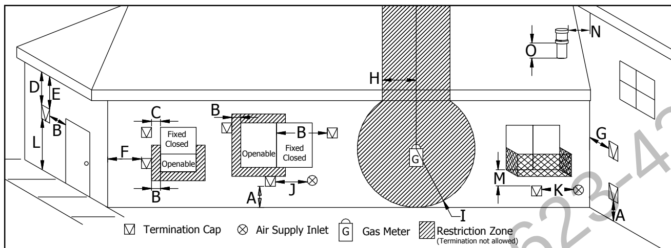
Figure 25. Vent Termination Restrictions, refer to Table 4.
