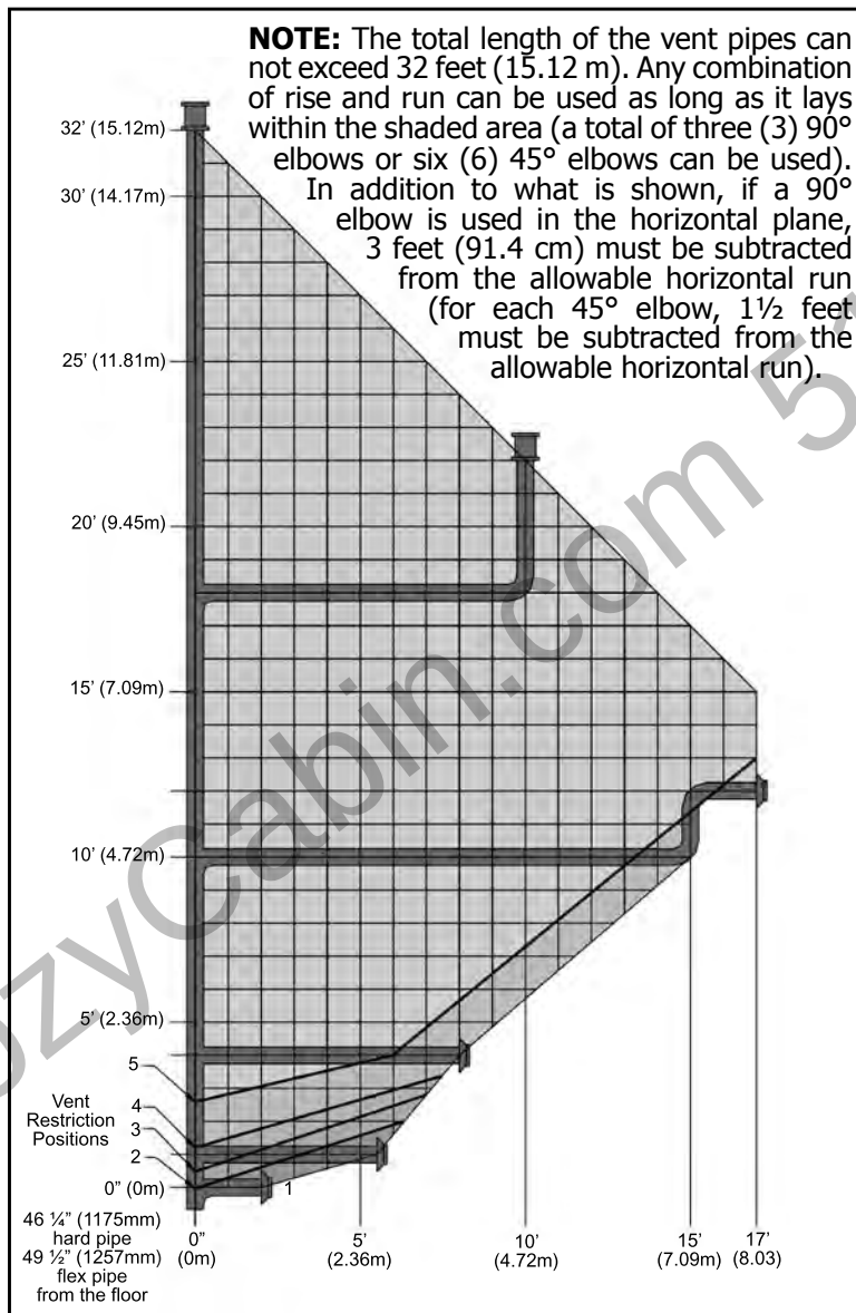
Figure 31. Possible Vent Configurations for Top Vented; Vertical and Horizontal Terminations.
