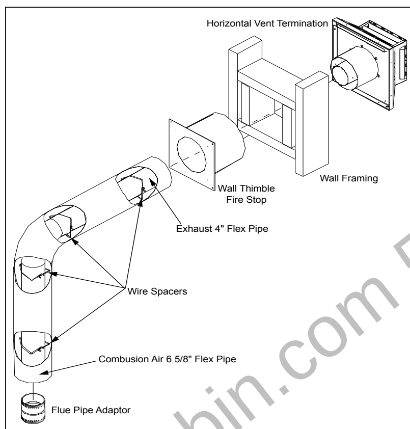
Figure 28: Installation of Fireplace Horizontal Vent Kit.
