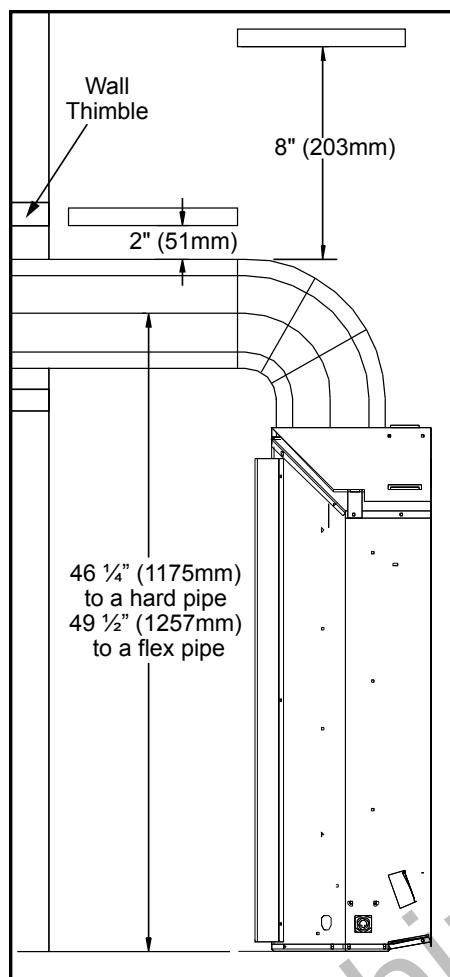
Figure 29. Vent Pipe Clearances.
