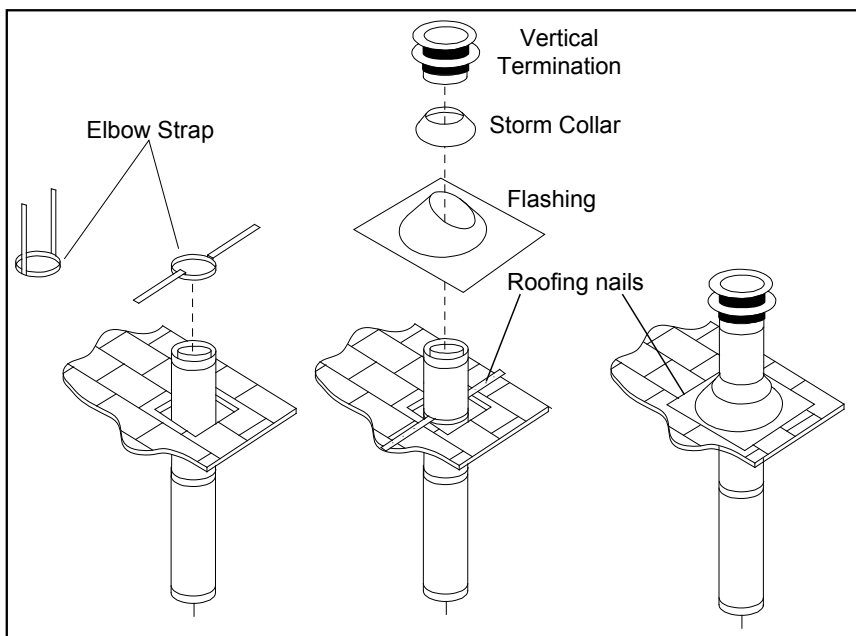
Figure 34. Vertical Vent Termination
