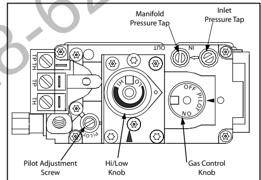
Figure 40. Fully Labeled Gas Valve.
