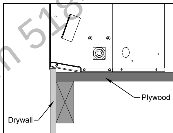
Figure 20. Drywall Facing Only Around The Retreat.
