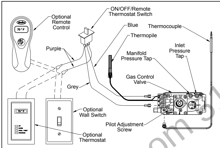
Figure 38. Wiring Diagram For Gas Valve.
