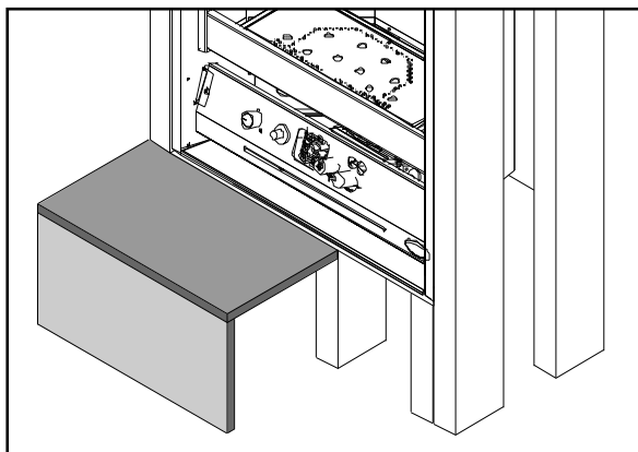
Figure 15. Raised Fireplace with Raised Hearth.
