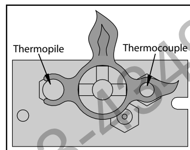
Figure 3. Pilot Flame
