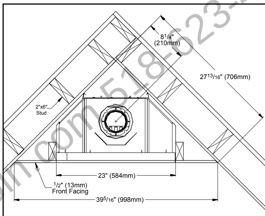
Figure 14. Dimensions for a corner installation.
