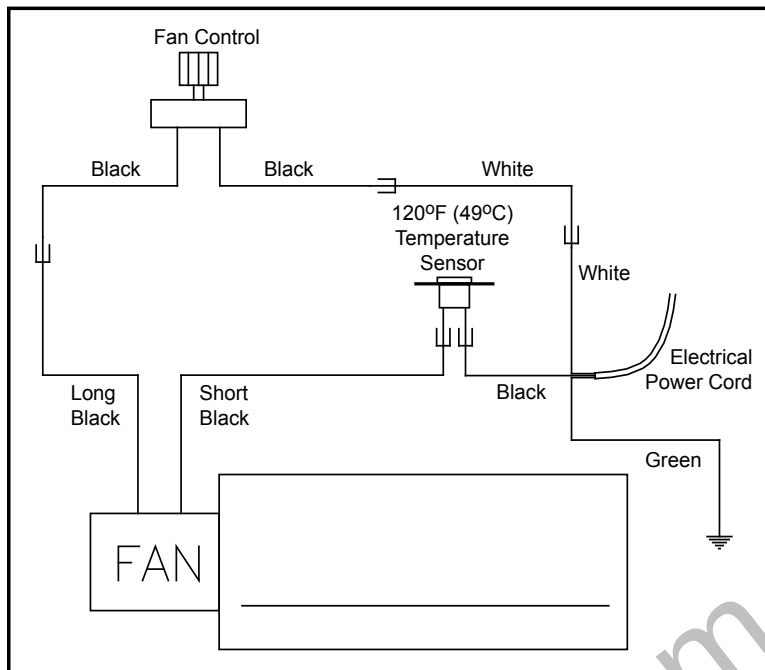
Figure 41. Wiring Diagram For Fan Control.
