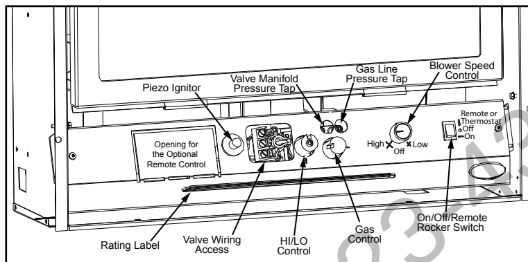
Figure 5. Control Panel
