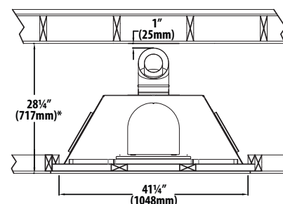
TYPICAL VERTICAL INSTALLATION REAR VENT
