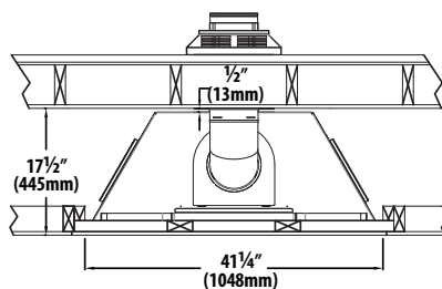
TYPICAL HORIZONTAL INSTALLATION TOP VENT
