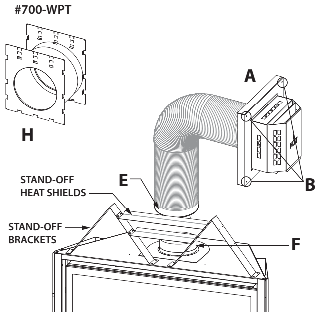
Figure 7.5, Installation and Assembly of #700-2 Series
