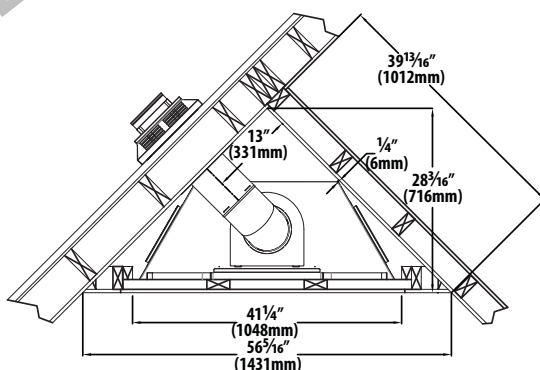
TYPICAL CORNER INSTALLATION TOP VENT
