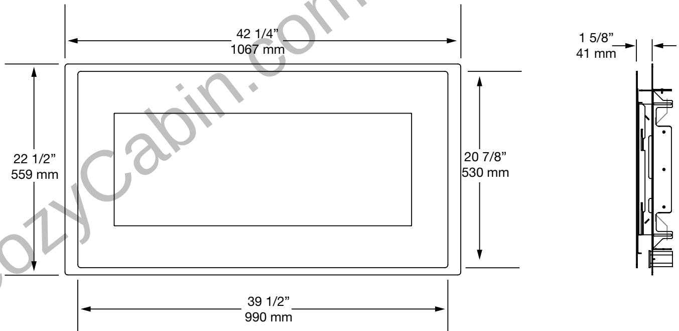
Figure 28: Esprit straight edge surround dimensions.
