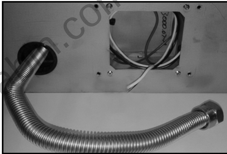
Figure 32: Electrical connection.
