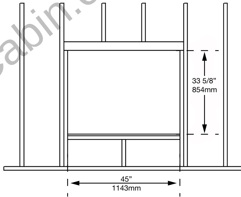
Figure 23: Framing dimensions.
