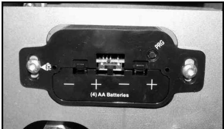
Figure 4: On-off switch.
