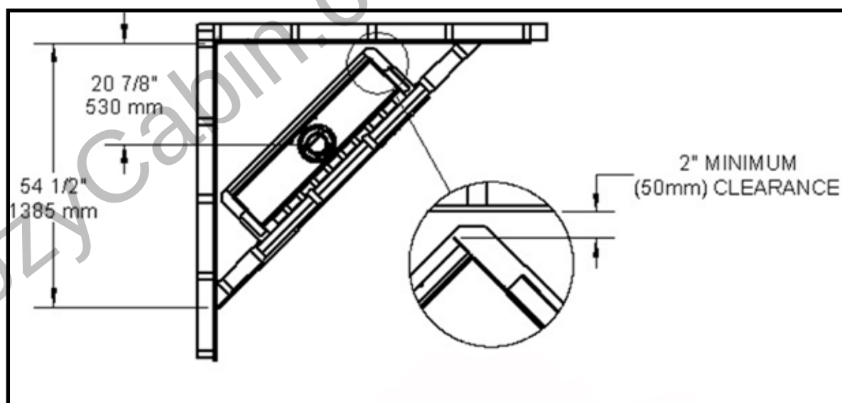
Figure 19: Minimum clearance corner framing.
